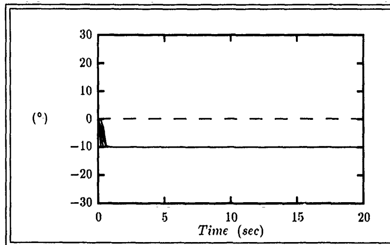
Figure G.129. \delta_{aL} Responses For Plants 1-6 to a 1 sec Duration 500^\circ/\text{sec} Yaw-Rate ( r ) Input to Design #1 (amplitude limited at +15^\circ and -10^\circ )
