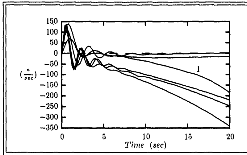
Figure G.128. r Responses For Plants 1-6 to a 1 sec Duration 500^\circ/\text{sec} Yaw-Rate ( r ) Input to Design #1
