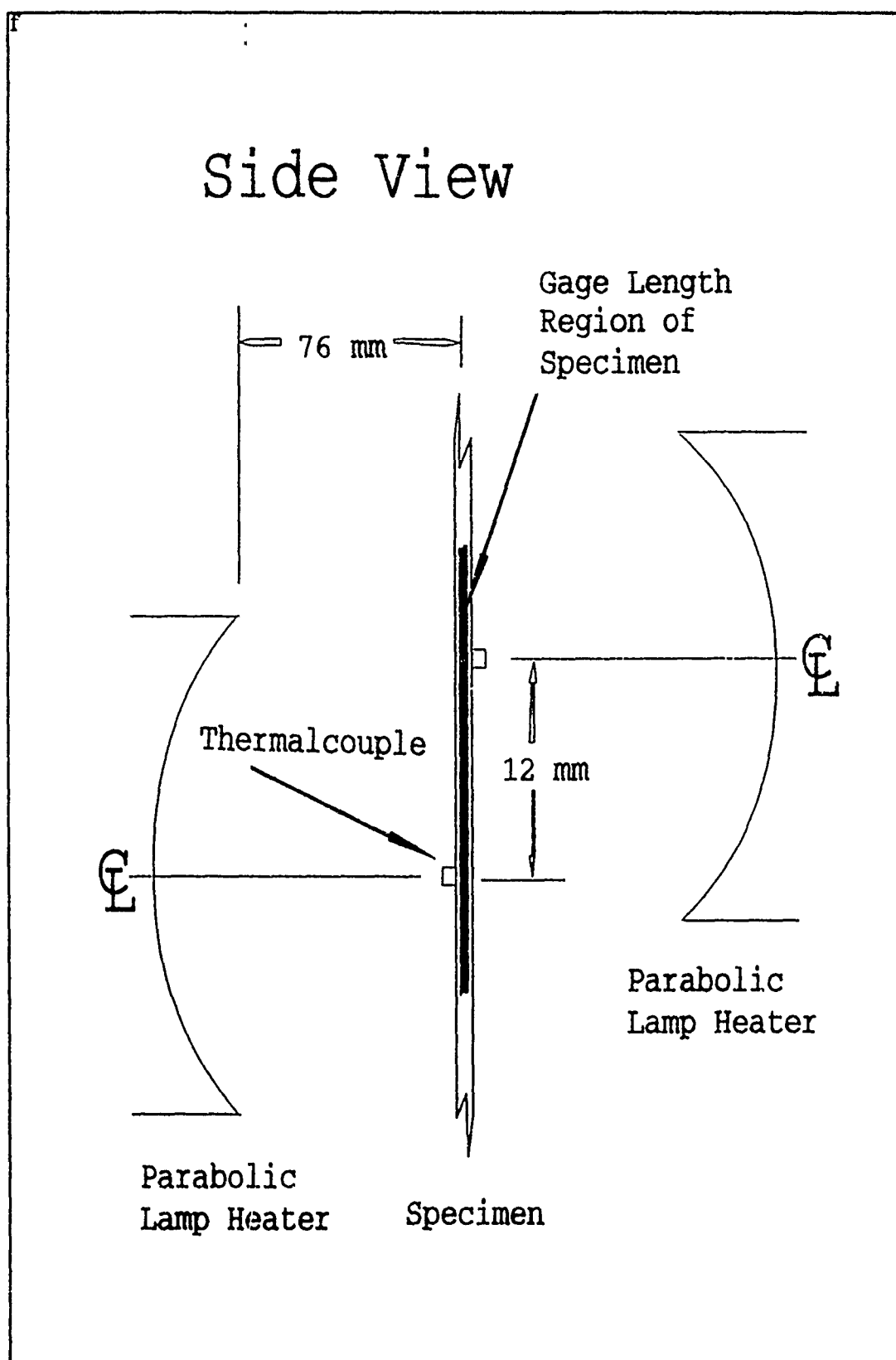
Figure 2. Thermocouple and Heater Placement Diagram
