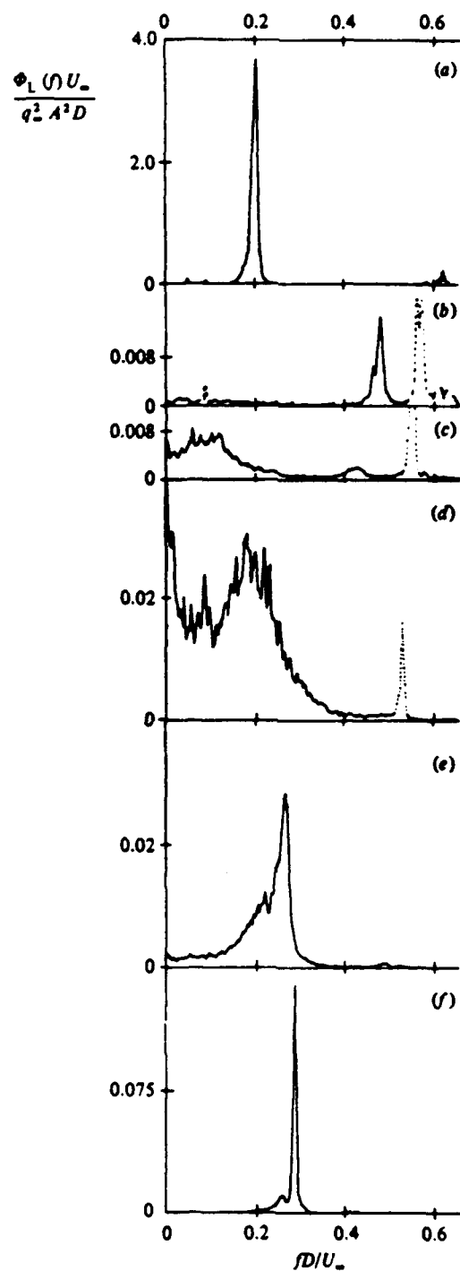
Figure 39. Power spectra of Lift Fluctuations. (a) Re = 1.3 \times 10^5 , (b) Re = 7.2 \times 10^5 , (c) Re = 1.9 \times 10^6 , (d) Re = 3.7 \times 10^6 , (e) Re = 5.9 \times 10^6 , (f) Re = 7.1 \times 10^6 (ref 22).
