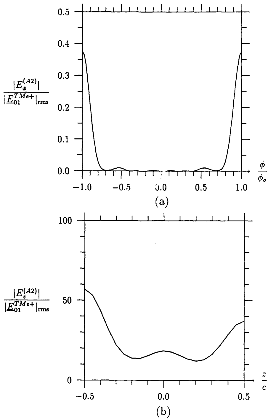
Fig. 8.11. The ratios (a) |E_{\phi}^{(A2)}|/|E_{01}^{TM_{e+}}|_{rms} and (b) |E_z^{(A2)}|/|E_{01}^{TM_{e+}}|_{rms} of the magnitudes of the \phi - and z -directed electric fields in the aperture A_2 to the root mean square value of the electric field of the incident TM_{01} wave in the circular cylinder when ka = 3.00 and L_3 = 0.5 \left[ \lambda_{01}^{TM} \right]_{ka=2.95} .
