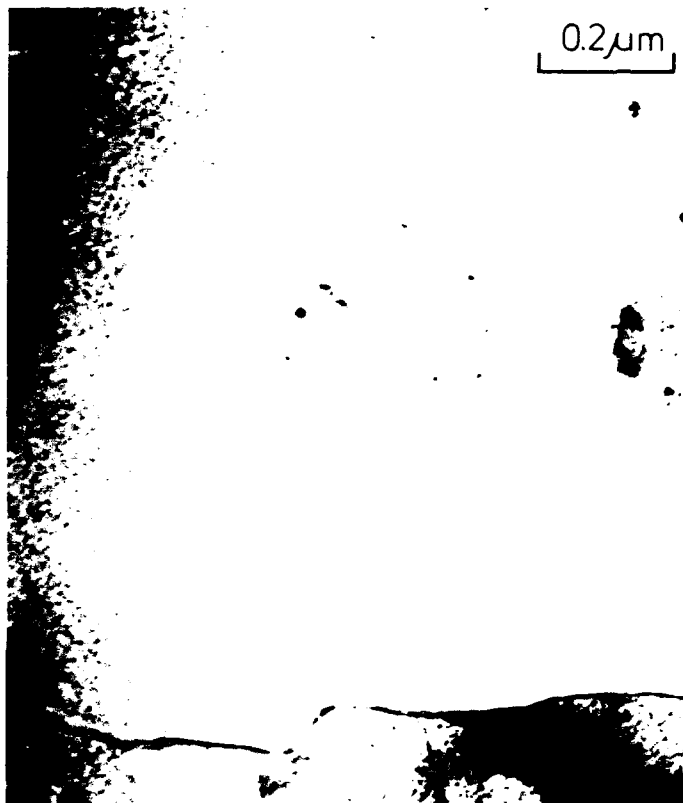
Fig 3 Transmission electron micrograph of vapour deposited RAE Alloy 72, as deposited at 170°C and aged at 260°C
