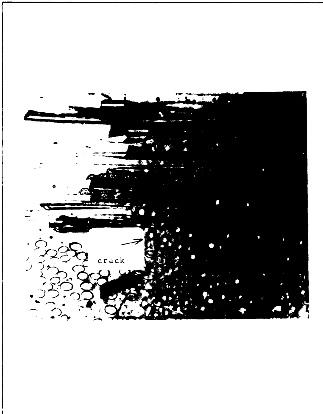
Figure 37 Matrix Cracking In 0^\circ Ply After 100 Cycles 13.0 KSI (90 MPa) Specimen
