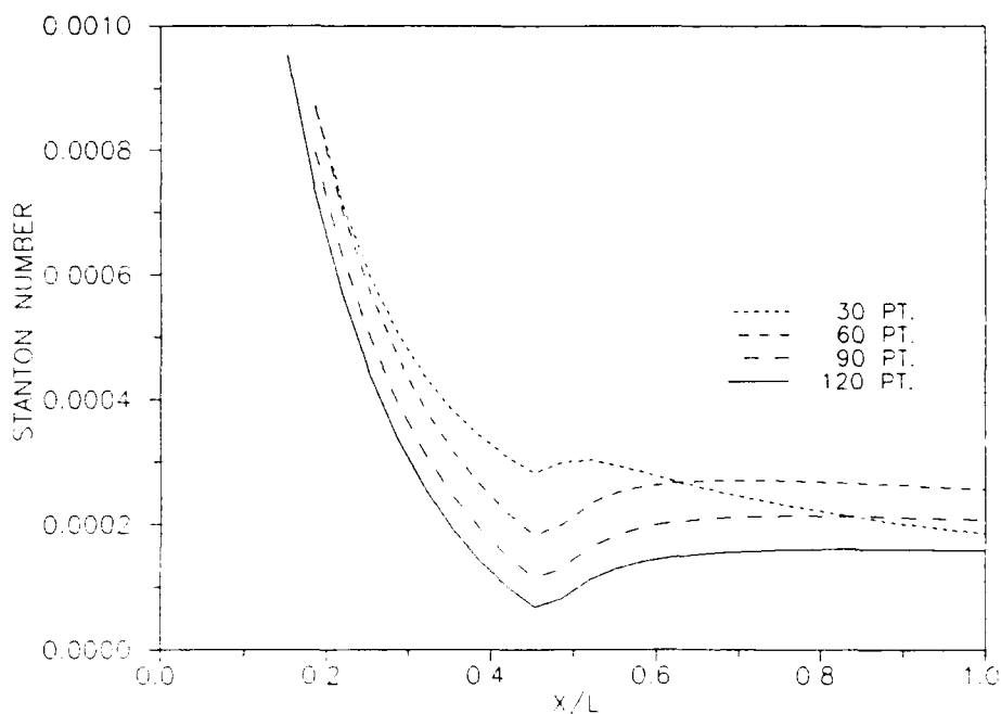
Figure 8. LMAX Effect on Stanton Number - Laminar Case
