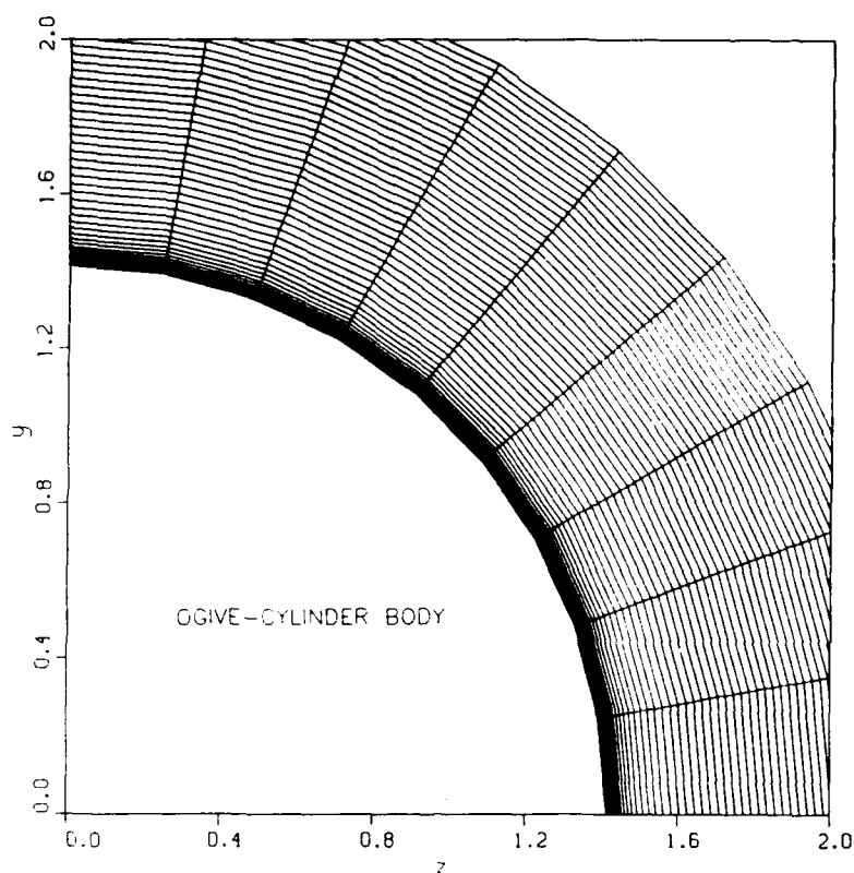
Figure 12. Grid Structure With Radial Clustering
