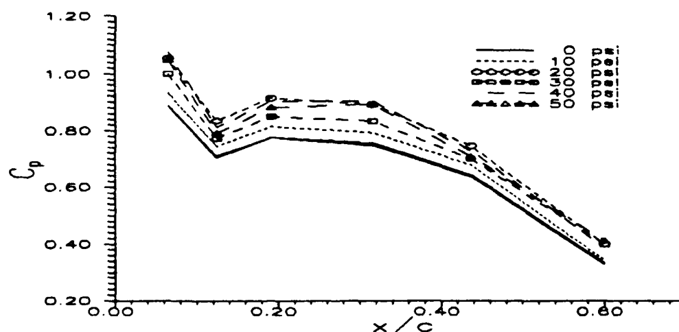
Figure 5.8a Pressure Coefficient Response Detail - Pressure Side
