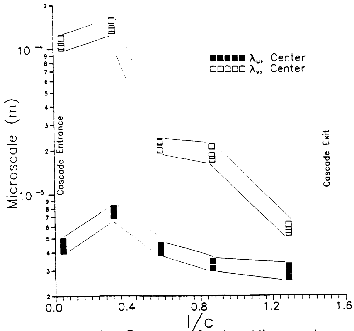
Figure 5.20 Passage Center Microscale
