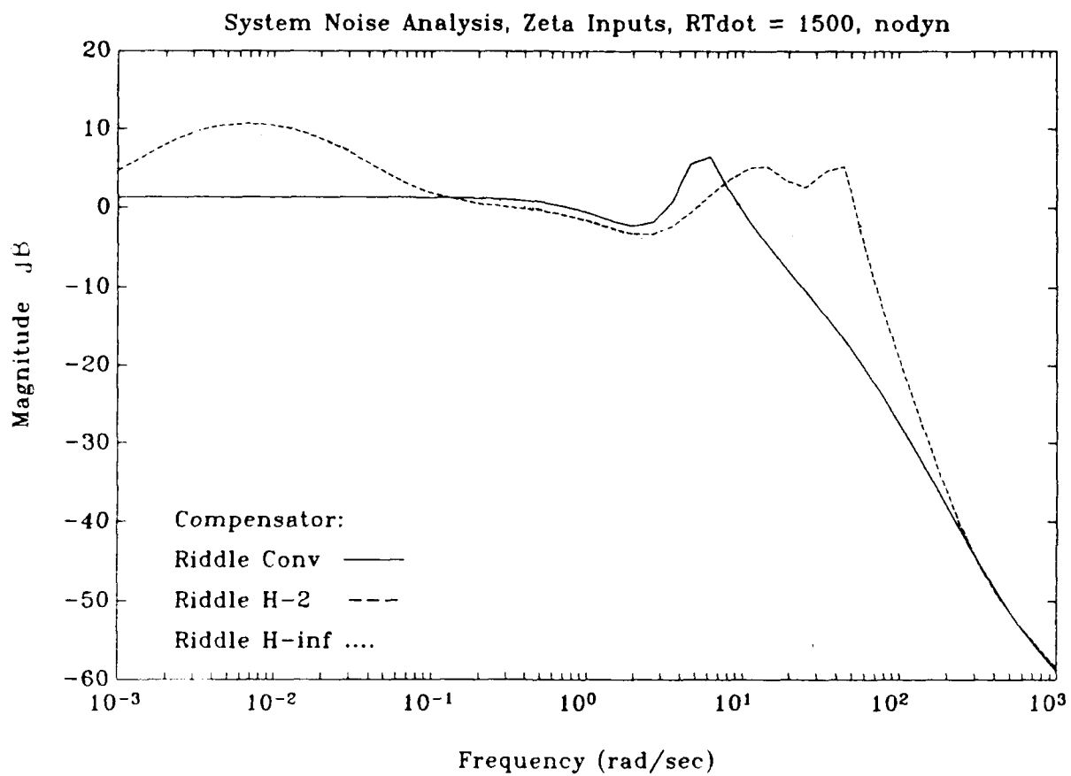
Figure 6.9 G_{\zeta} Singular Value Plots without Unmodelled Dynamics
