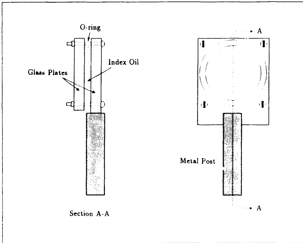
Figure 4.11. Optical Feedback Compensator Design
