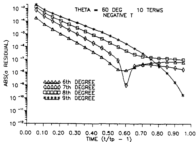
Figure 10c. Absolute Value of the a Residual vs. Negative T for a Transfer Angle of 60^\circ Using 10 Terms with the Coefficients Calculated Using Polynomials of Degree 6 - 9
