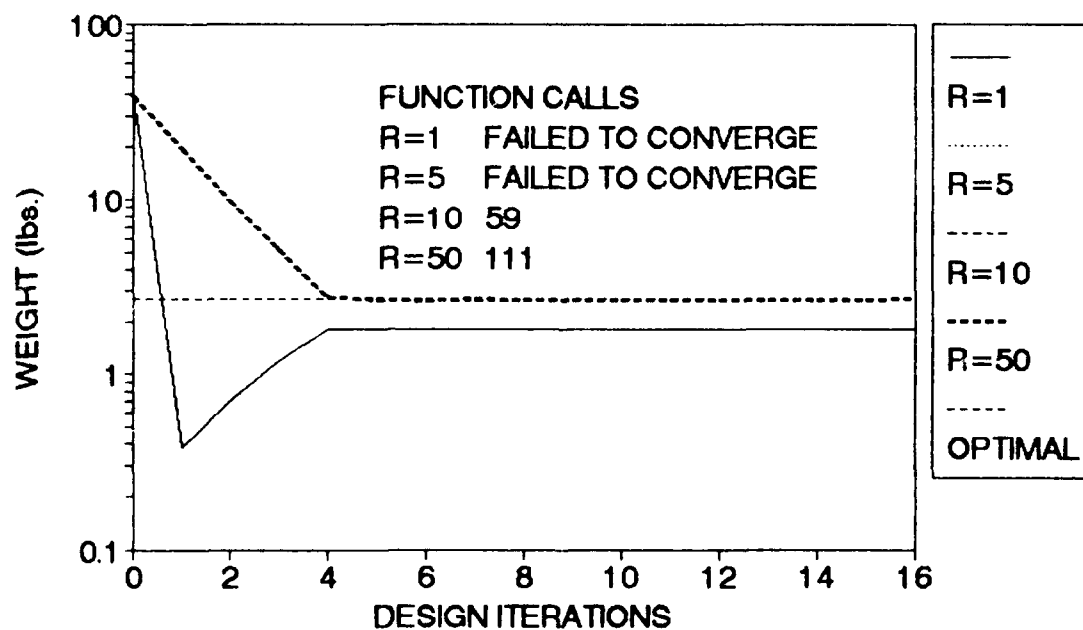
Fig. 12 - Case No. 4 CSD - Three-Bar Truss
