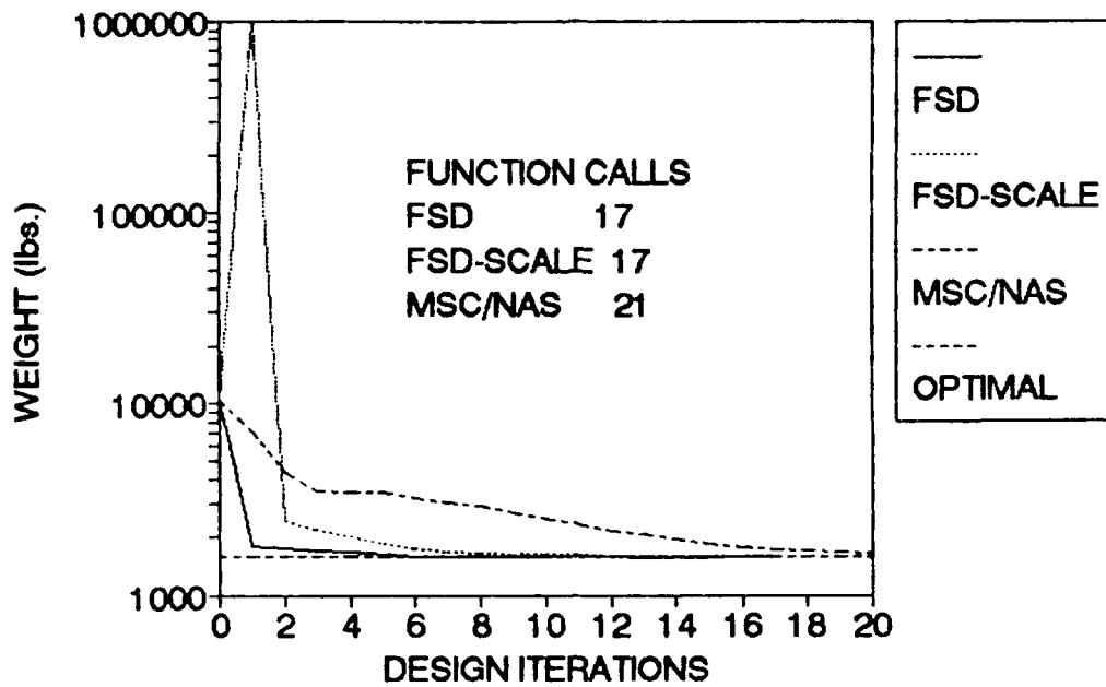
Figure 31. Case No. 3 FSD and MSC/NASTRAN - Ten-Bar Truss
