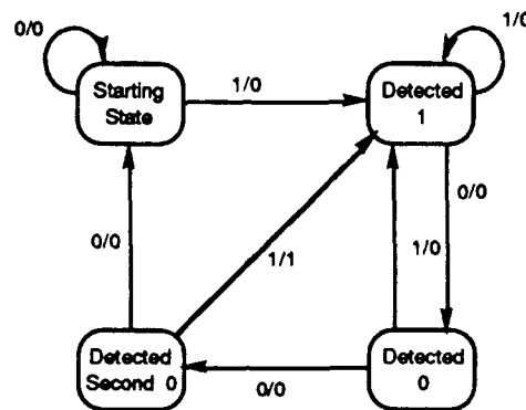
Figure 5.2. Sequence Detector.
