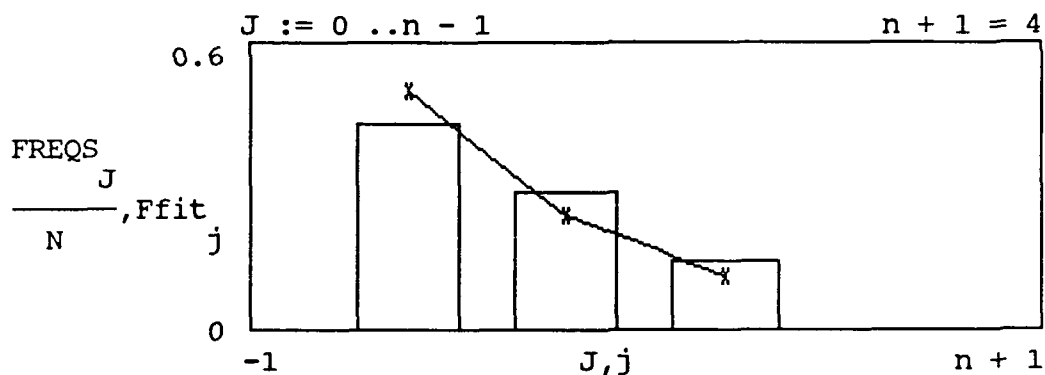
Figure C-1. Histogram of Data
