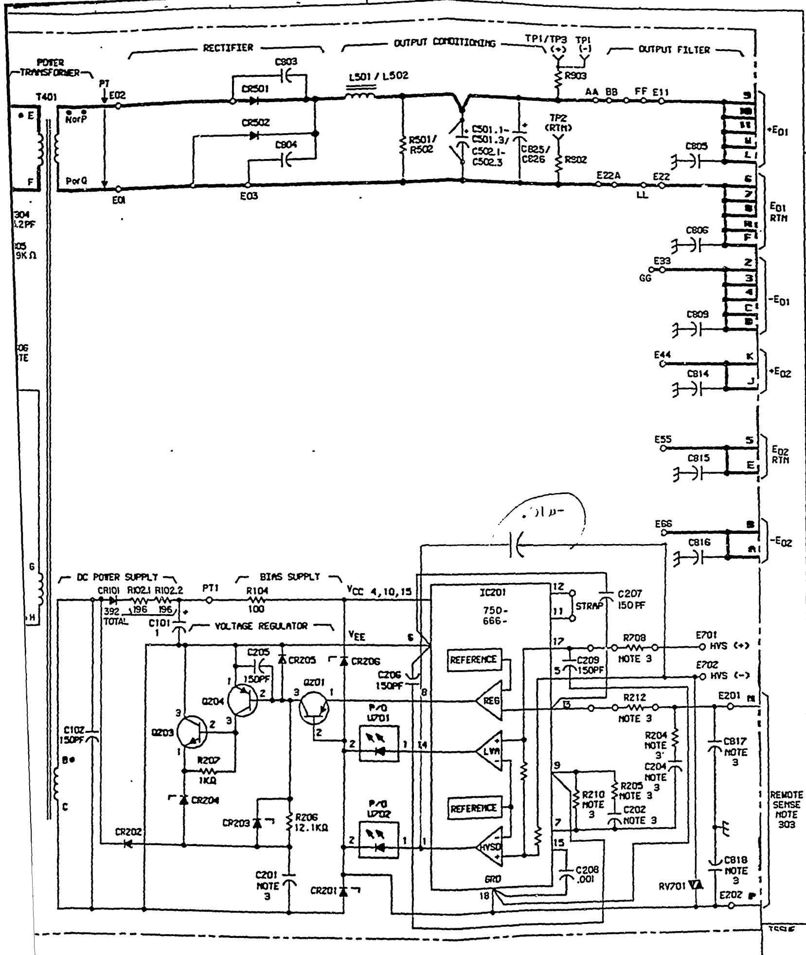
Figure 8. Schematic of 140L1 circuit pack, with modifications circled
