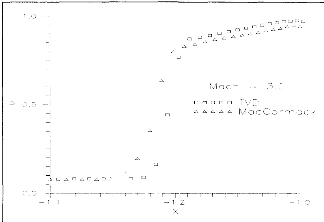
Figure 7. Pressure Along the Line of Axisymmetry, Second-Order TVD and MacCormack Schemes, Mach = 3.0
