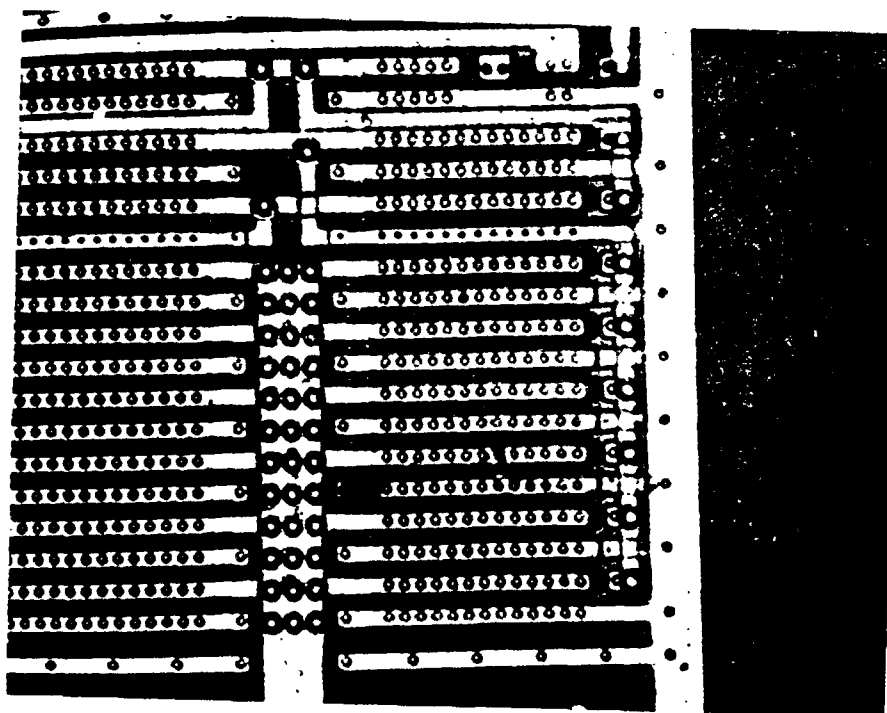
Figure 72 SN056, Pin 31: Output Pad Short
