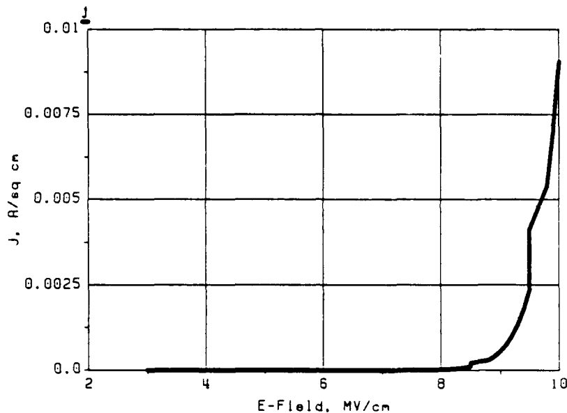
Figure 1 Injected Current Density as a Function of E-Field
