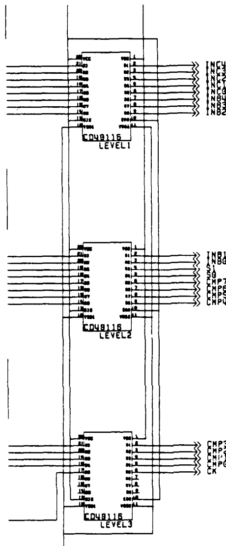
Figure 64 Life Test Board Level Shifting
