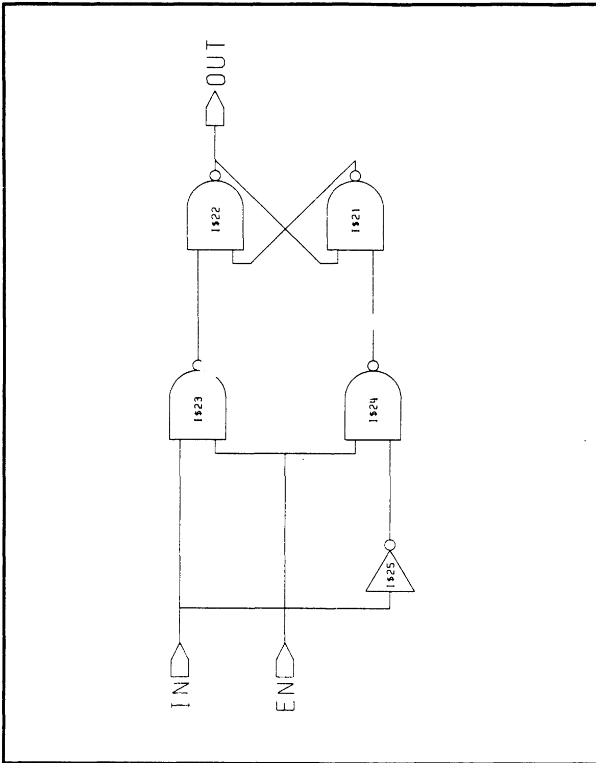
Figure 92 RLOS Test Vehicle (B,C) Latch
