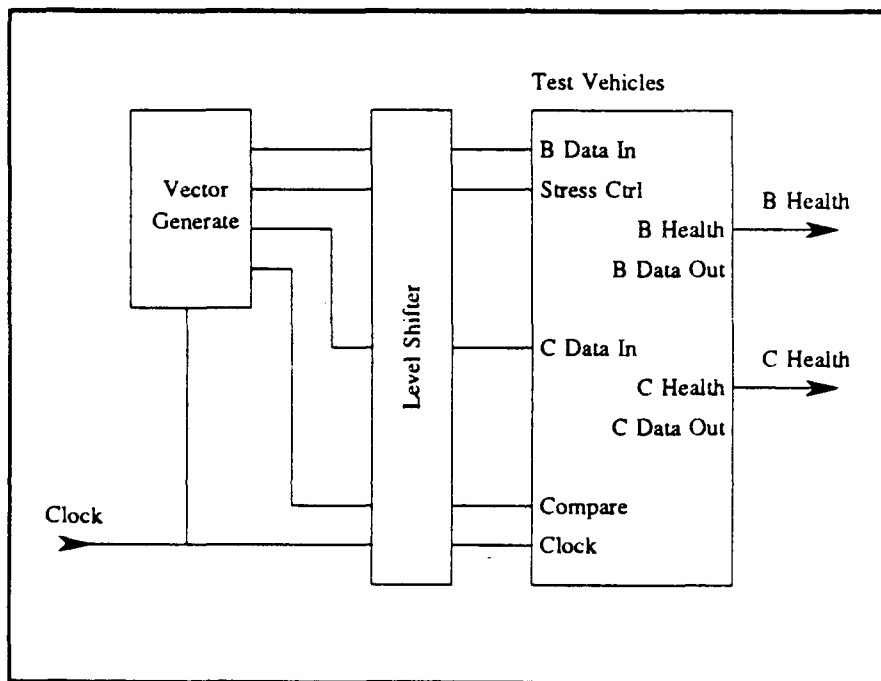
Figure 62 Life Test Board Functional Block Diagram
