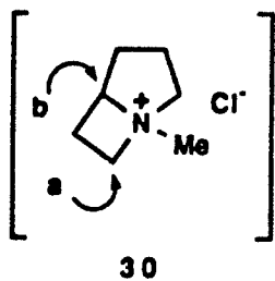
Scheme 7
