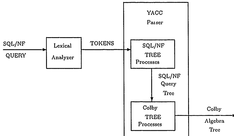
Figure 4.1. Query Tree Process
