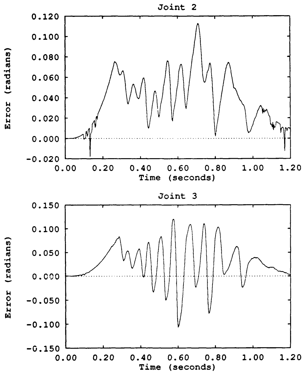
Figure 3.4. PD Feedback Tracking Error
