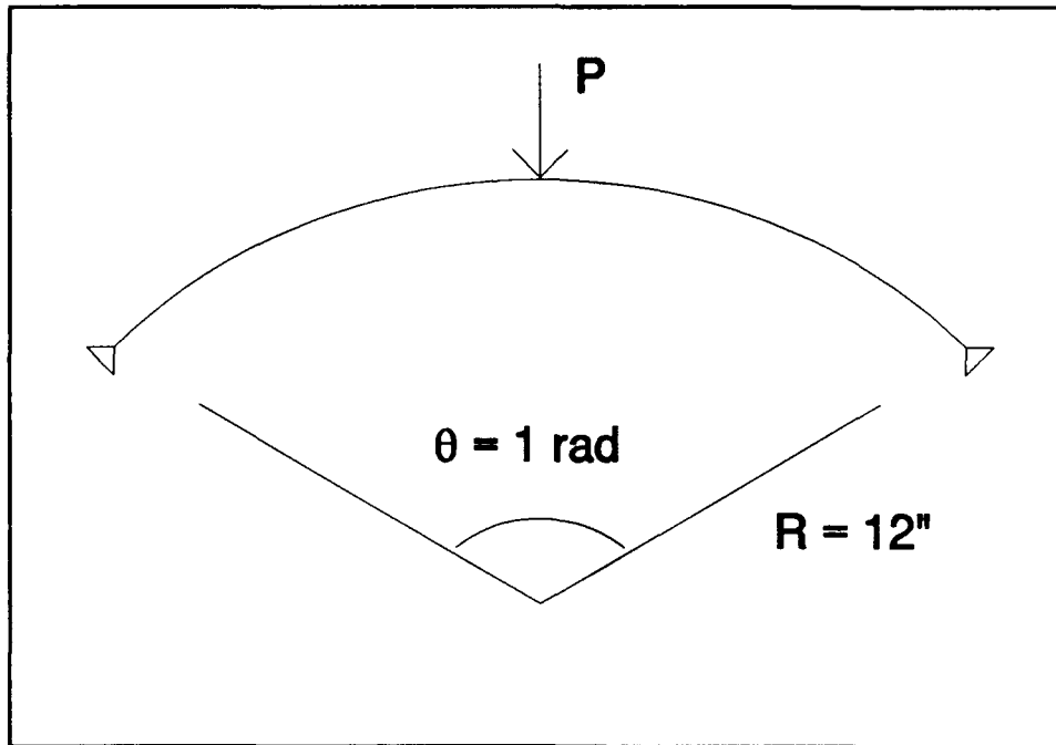
Figure 3-11. Laminated Arch
