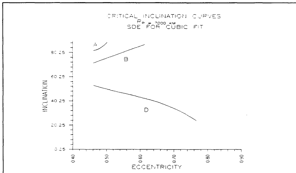
Figure 36. Critical Inclination Curves: Periapse Radius = 7000 Km, Cubic Data Fit
