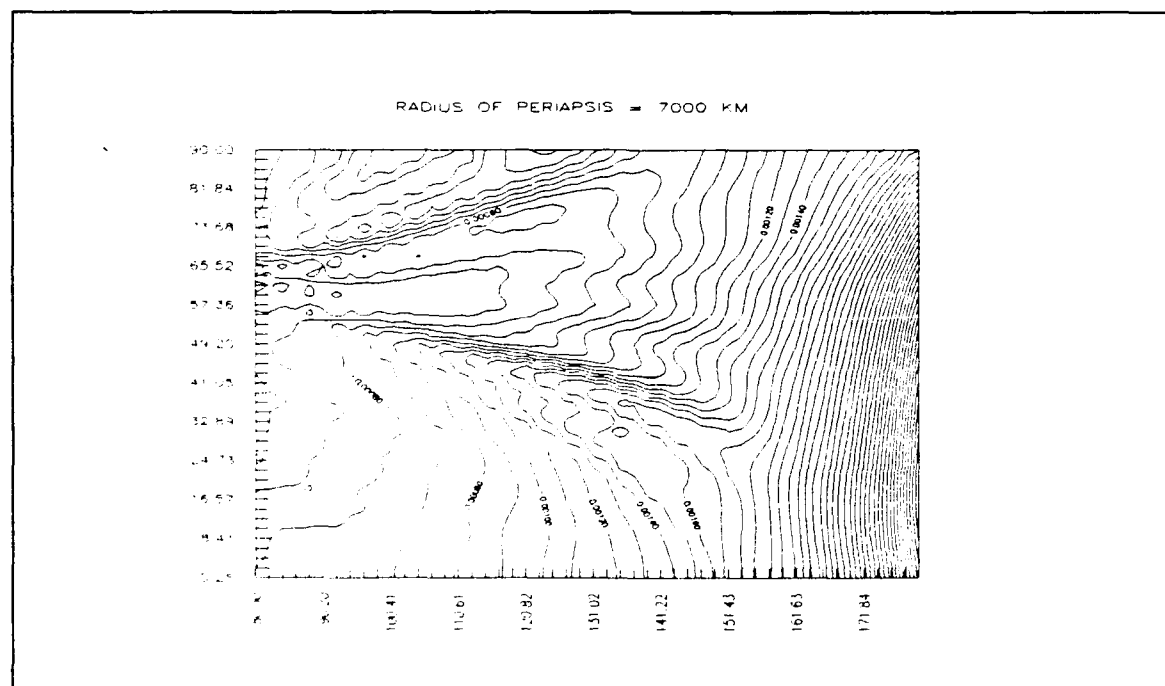
Figure 37. 2-D Contour Plot: Periapse Radius = 7000 Km, Cubic Data Fit
