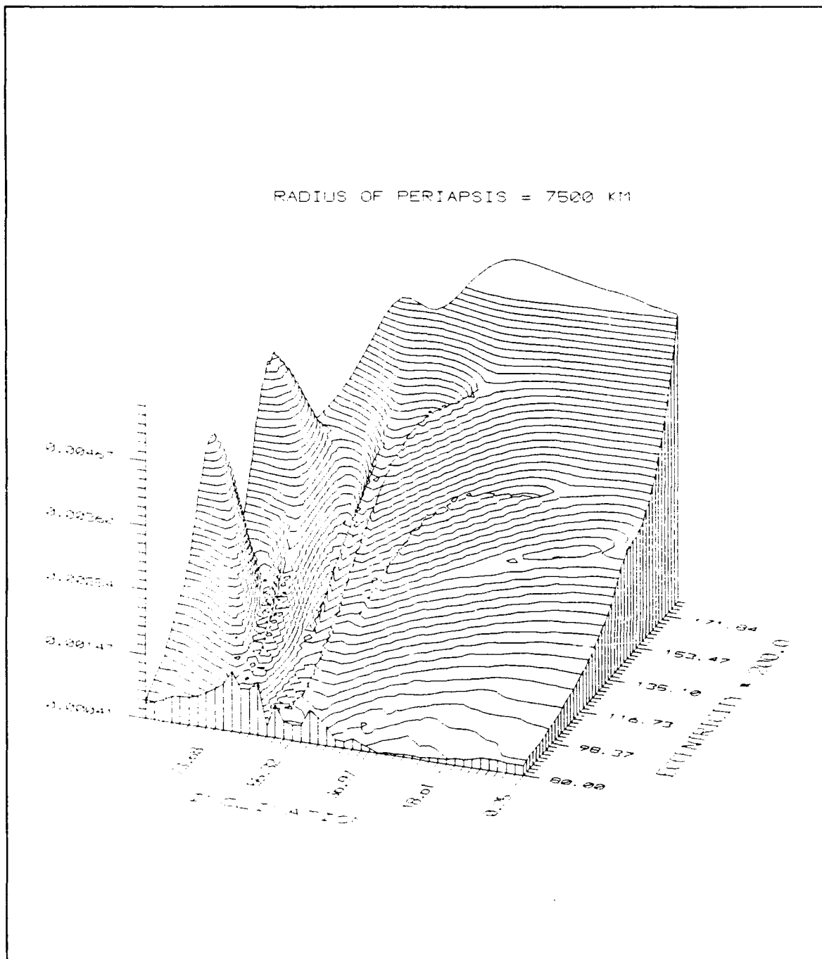
Figure 13. Standard Deviation in Eccentricity vs Inclination and Eccentricity: Periapse Radius = 7500 Km, Linear Data Fit
