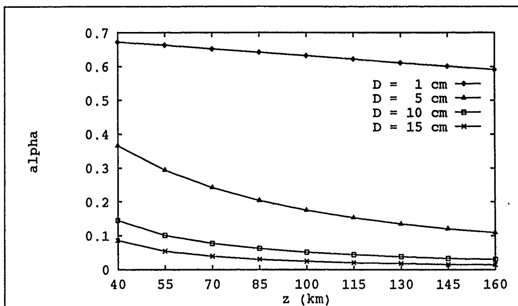
Figure 14. Alpha Versus Path Length with Varying Aperture Size: h = 5000\text{ m}
