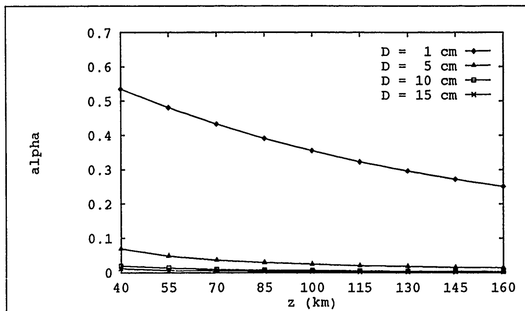
Figure 15. Alpha Versus Path Length with Varying Aperture Size: h = 8750\text{ m}
