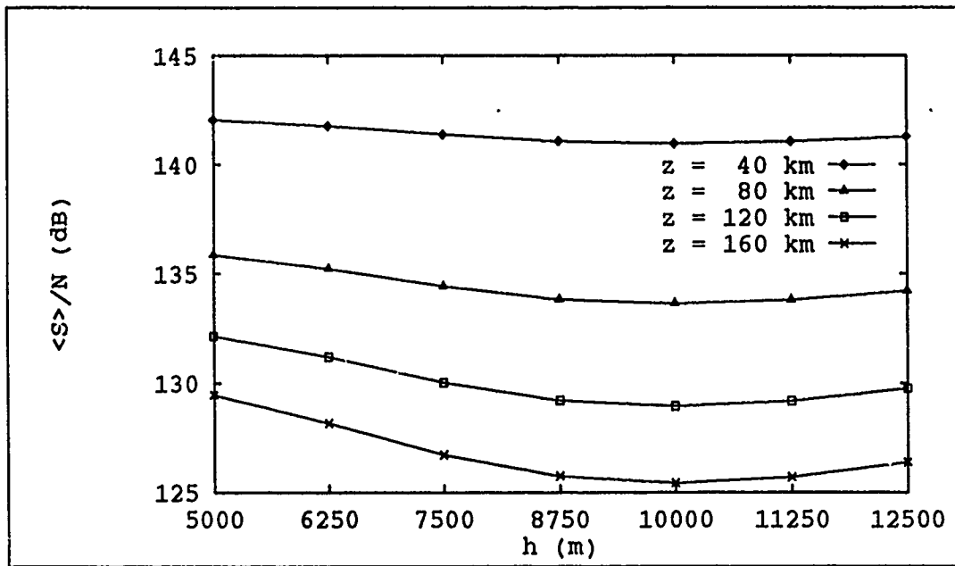
Figure 24. Signal-to-Noise Ratio Versus Altitude with Varying Path Length - D = 1 cm
