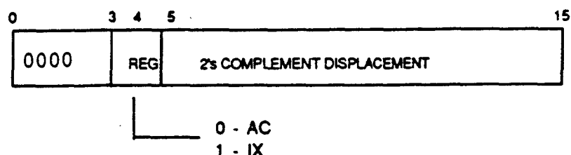
FIGURE 5-12. ADD Instruction
