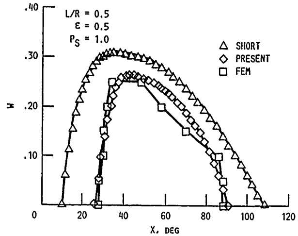
Fig. 16. - Cavity shape.
