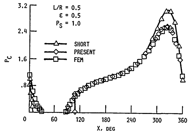
Fig. 17. - Centerline pressure.
