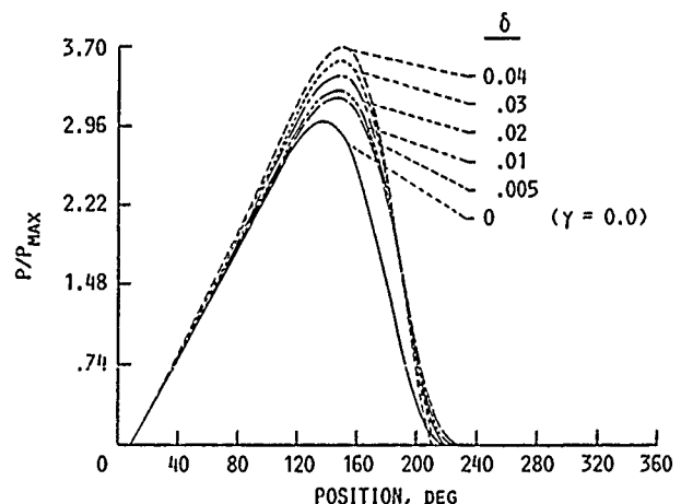
Fig. 5. - Pressure profiles in shear thickening fluid ( \gamma = -0.1 ).
