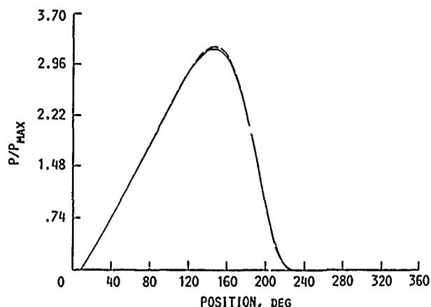
Fig. 8. - Pressure profiles at \gamma = -0.1 .
