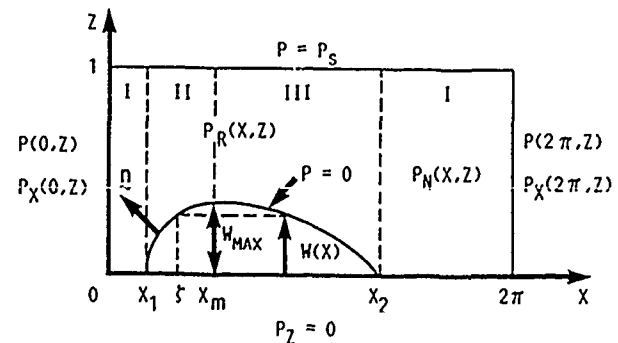
Fig. 15. - Bearing surface.
