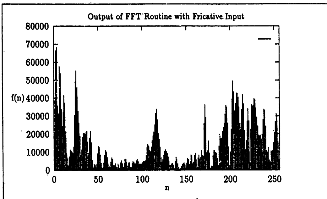
Figure 14. FFT Output with Fricative Input
