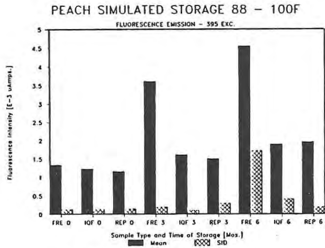
Figure 3. Fluorescence Emission.
