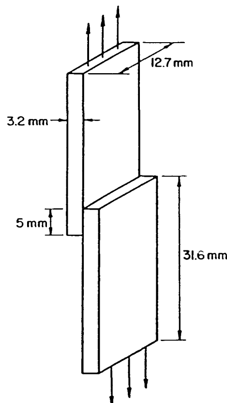
Fig. 29. Lap shear joint method used to test weld strength of polymers (Kline and Wool).
