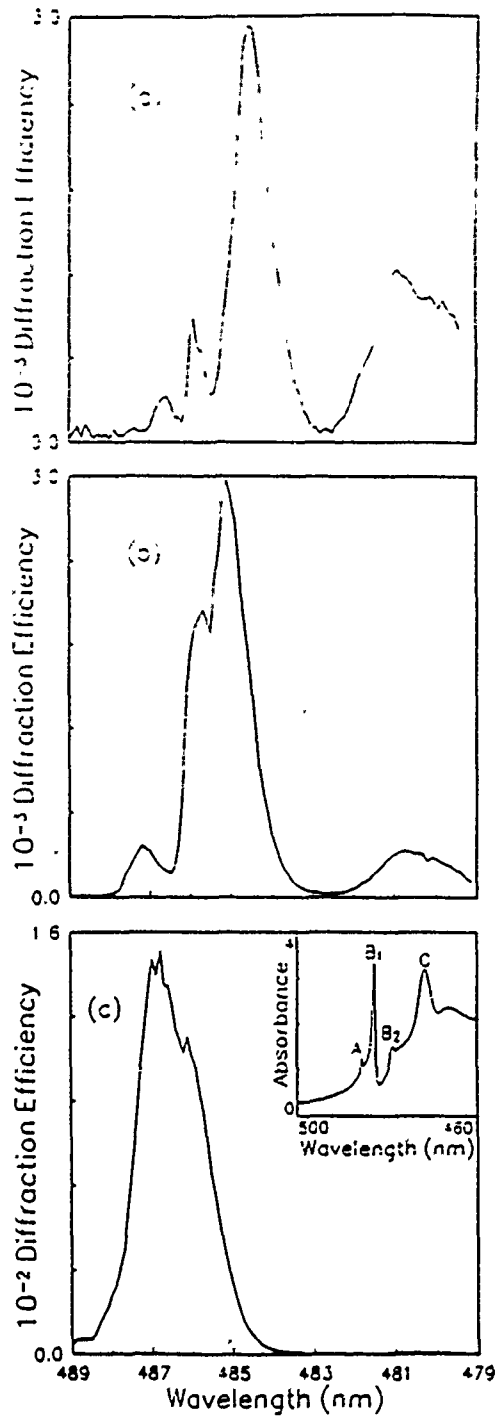
Figure 3. Experimental diffraction efficiency spectra for CdS. Sample thickness was 5 \mu\text{m} . Peak pulse energies were (a) 4 nJ, (b) 40 nJ, (c) 400 nJ. Inset to (c) shows the linear absorption spectrum for a sample of CdS less than 0.2 \mu\text{m} thick. Sample temperature for DFWM and absorption measurements was 30 K. Spot radius w_0 = 37.5 \mu\text{m} . Beam internal angle \cong 0.5^\circ .
