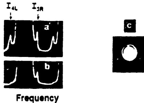
Fig. 5. I_{4L} and I_{3R} spectra with the cone (a) unblocked and (b) blocked, showing that almost all of I_{4L} goes into the cone. (c) Photograph of cone with the \cong 100\times more intense center overexposed.
