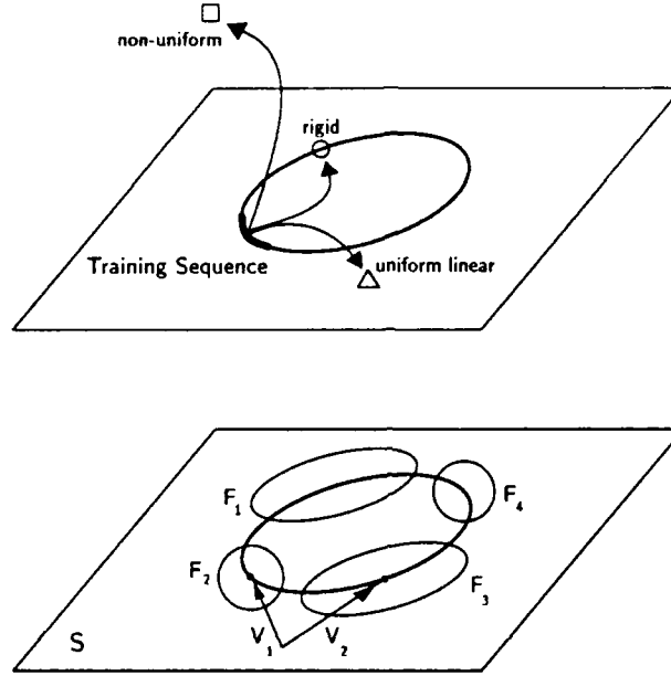
Figure 12: Top: An illustration of the three transformation categories explored in the DEF experiments (the relevant mathematics appear in [31]; see also [8]). A novel view related to the training views by a rigid rotation is indicated schematically by the small circle lying on the ellipse that represents the quadratic constraint curve within the space of all possible views of the training object. Another view, which is the result of a uniform linear but not necessarily rigid transformation, is represented by the small triangle. A third view is obtained through a nonuniform deformation and is shown by the square which lies outside the linear space of all possible views. Bottom: A schematic illustration of two ways to represent objects by multiple views. The CLC+ scheme covers the space of all possible views (rigid transformations) of the object by imposing a nonlinear constraint (boldface ellipse) on the linear space S spanned by a small number of training views ( V_1 and V_2 ). The HyperBF scheme approximates the same subspace by a larger set of basis functions ( F_1 through F_4 ), which can be nonradial and can extend outside the linear space S .
