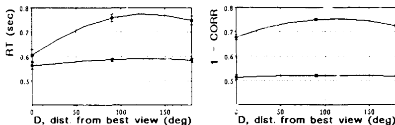
Figure 6: Experiment CV: Left : Regression analysis of the subjects' response times. Define the best view for each object as the view with the shortest RT. If recognition involves rotation to the best (canonical) view, RT should depend monotonically on D = D(\text{target}, \text{view}) , the distance between the best view and the actually shown view. Right : Regression analysis of the CLF model's performance. The plotted variable is 1 - \text{CORR} , since high values of CORR are analogous to short response times. (The decrease in RT or CORR at D = 180^\circ is due to the fact that for the wire-frame objects used in the experiments the view diametrically opposite the best one is also easily recognized.) For both human subjects and the model, the dependence is clear for the first session of the experiment (upper curves), but disappears with practice (second session - lower curves).
