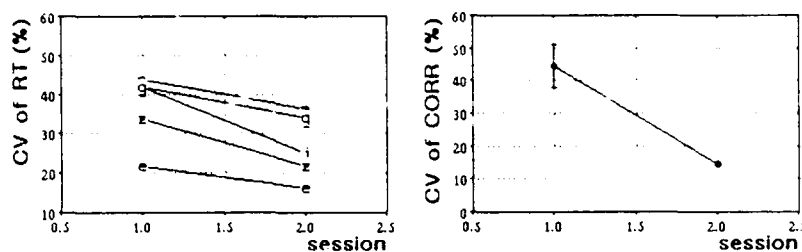
Figure 5: Experiment CV: Left : Performance of five human subjects. The variation of response time over different views of an object (an estimate of the strength of the canonical views phenomenon) decreases with practice. Right : Performance of the CLF model in a simulated experiment was similar to that of human subjects. The performance measure CORR is defined as the correlation between the input and a stored representation and serves as an analog of the response time [9]. In this and other figures the error bars denote \pm 1 standard error of the mean (the bars are too small to be visible in the left panel).
