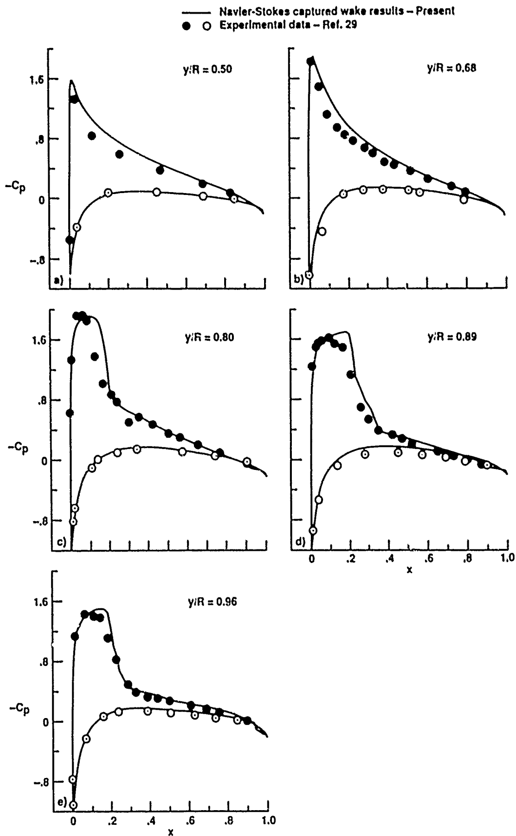
Fig. 4 Comparison of surface pressures for a lifting hovering rotor; M_{tip} = 0.794 , \theta = 12^\circ , and Re = 3.55 \times 10^6 .
