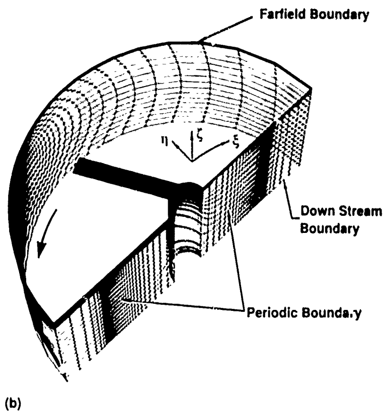
Fig. 1 Coarse C-H cylindrical grid topology for a two-bladed rotor; a) view in the plane of the rotor, and b) isometric view showing the grid boundaries for a single blade.
