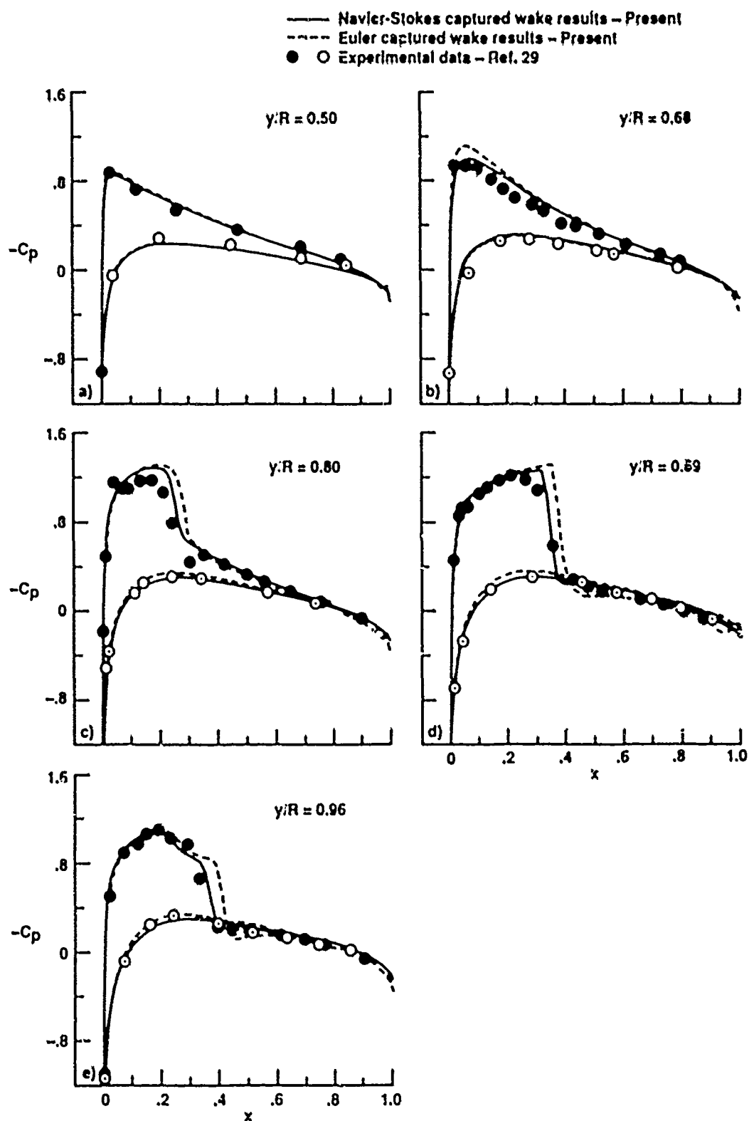
Fig. 10 Comparison of surface pressures for Euler and Navier-Stokes solutions; M_{tip} = 0.877 , \alpha = 8^\circ , and Re = 3.93 \times 10^6 .
