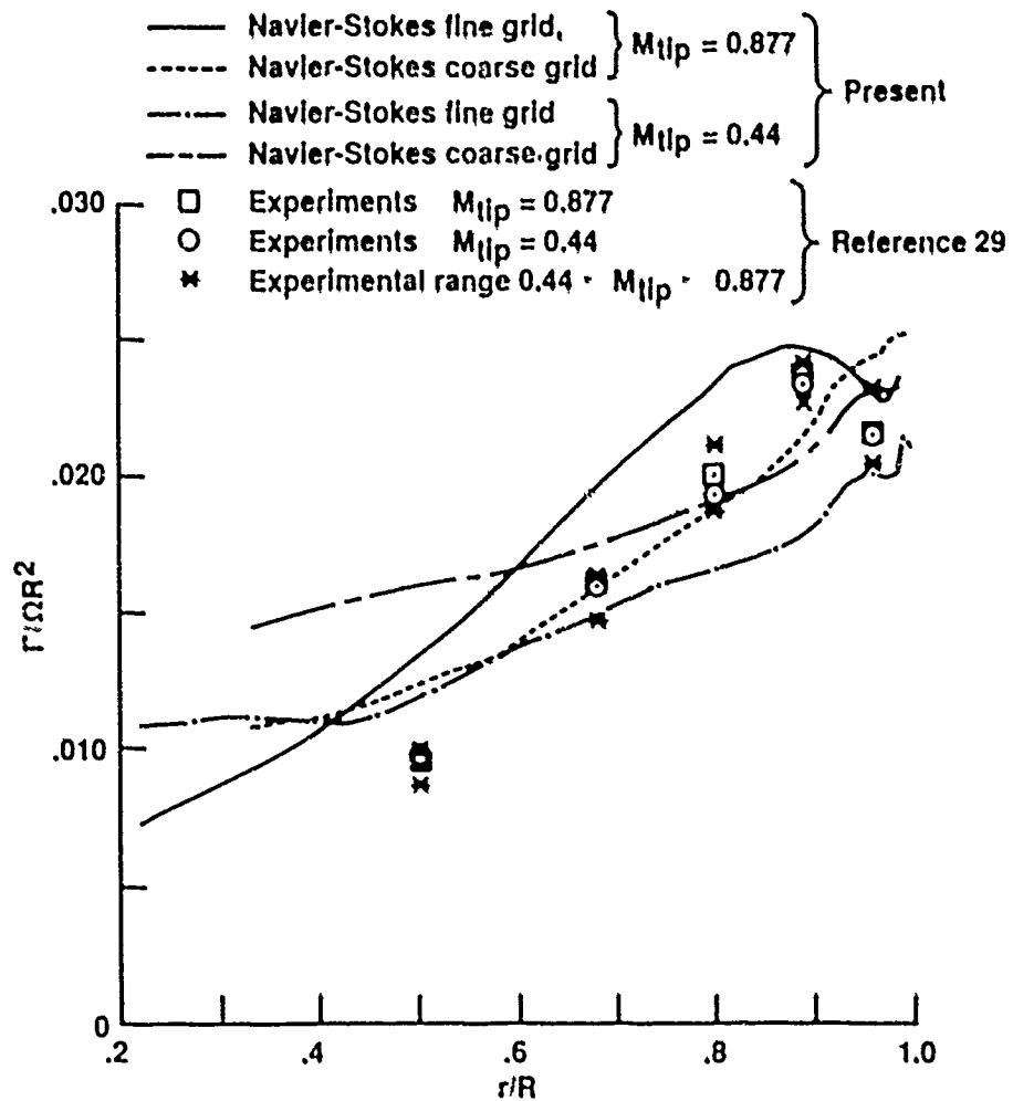
Fig. 6 Comparison of bound circulation distribution for the case of collective pitch \theta = 8^\circ with tip speeds of M_{tip} = 0.44 and 0.877 .
