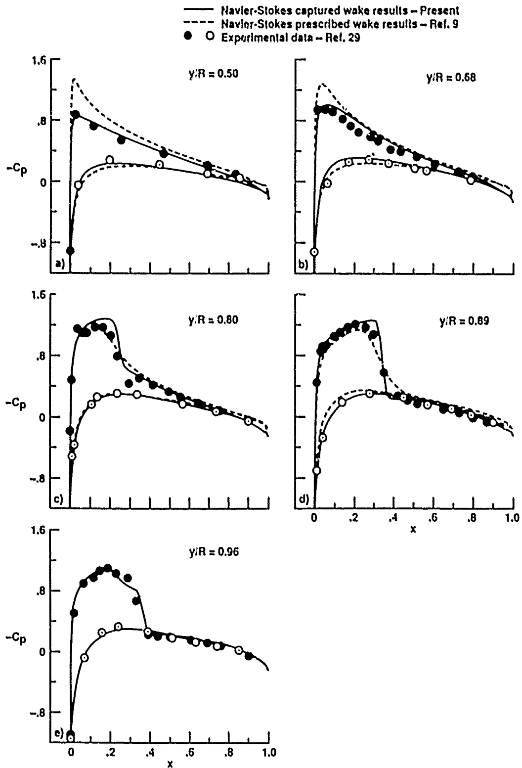
Fig. 3 Comparison of surface pressures for a lifting hovering rotor; M_{tip} = 0.877 , \theta = 8^\circ , and Re = 3.93 \times 10^6 .
