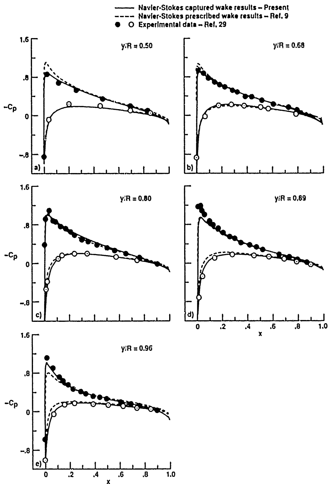
Fig. 2 Comparison of surface pressures for a lifting hovering rotor; M_{tip} = 0.44 , \theta = 8^\circ , and Re = 1.92 \times 10^6 .
