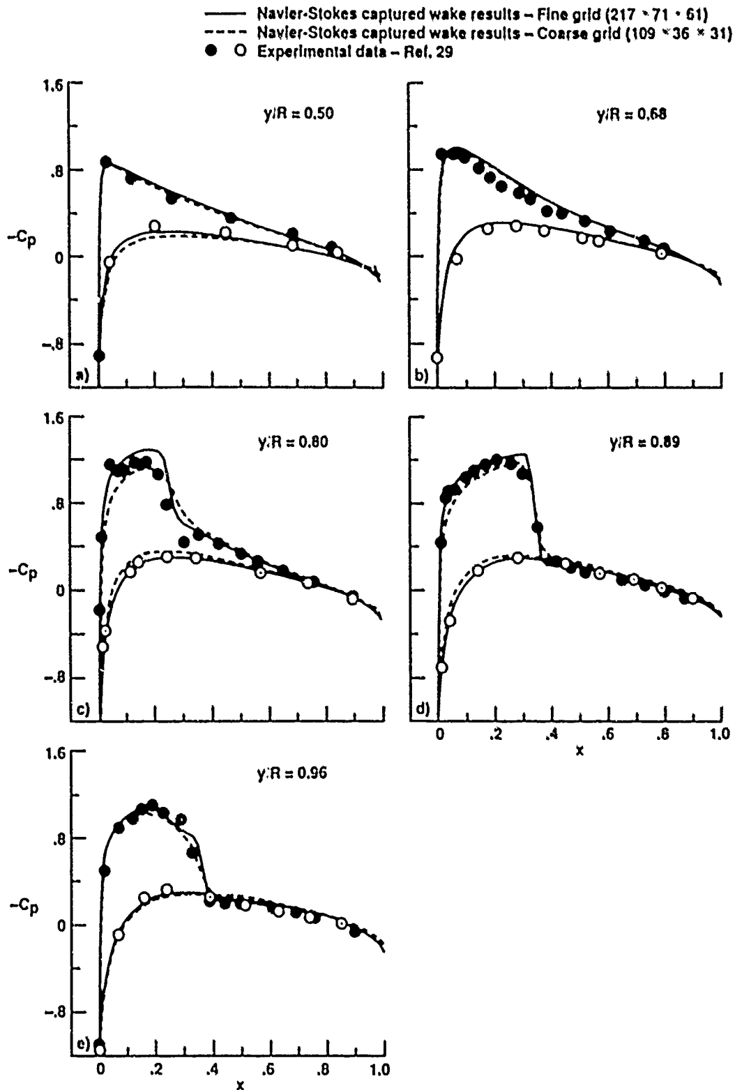
Fig. 9 Comparison of surface pressures with coarse and fine grids for the case of M_{tip} = 0.877 , \theta = 8^\circ , and Re = 3.93 \times 10^6 .
