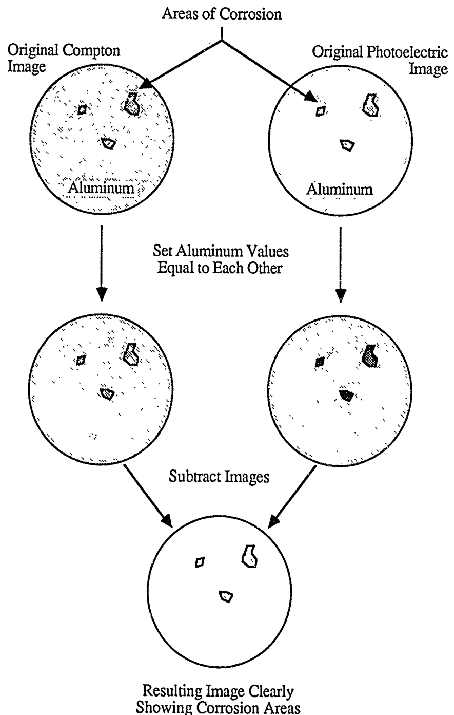
Figure 1 Dual-Energy Image Subtraction Process
