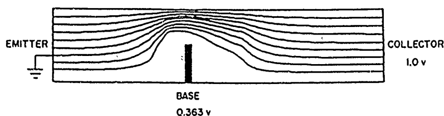
Figure 4 Current Flow Inside the Device
