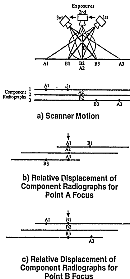
Figure 2 Schematic of Data Imaging for Laminography
