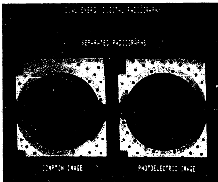
Figure 5 Compton and Photoelectric Images of Antenna Panel
