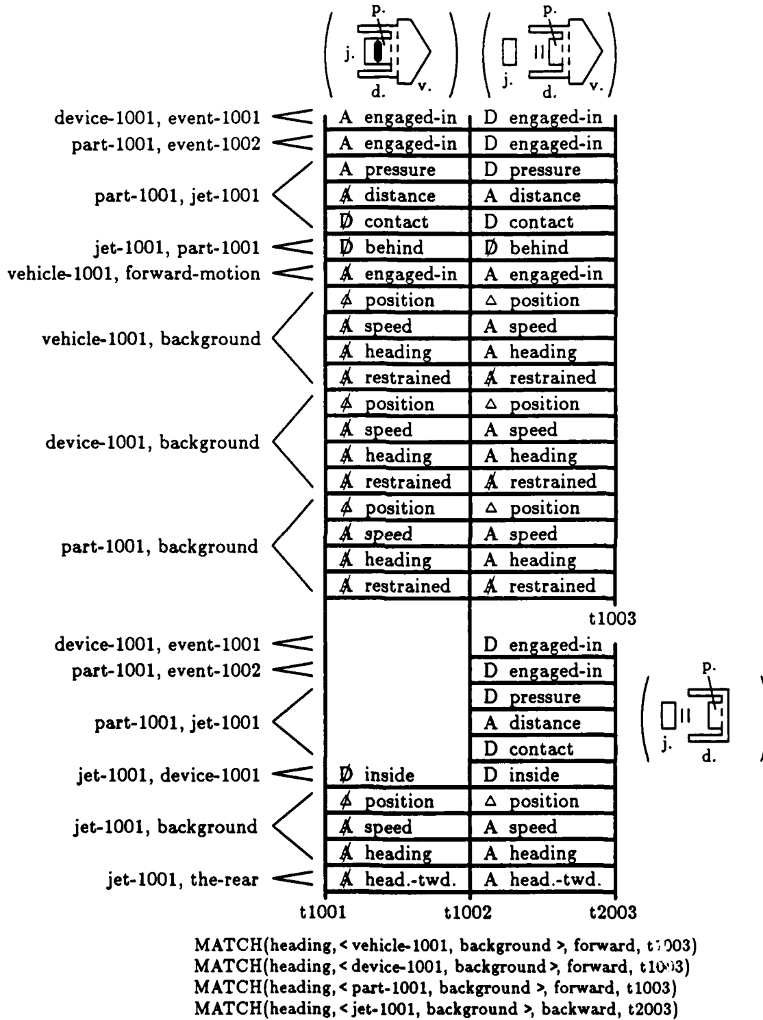
Figure 7: Composite trace for the rocket example.
