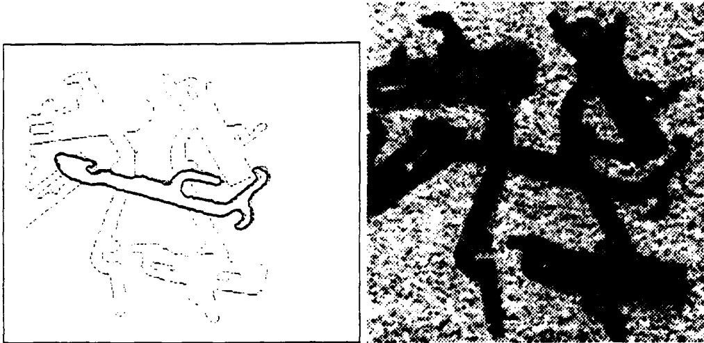
Figure 20: A real example. On the left is displayed the leading hypothesis. The model contour has been transformed and plotted over the image contours, indicating the pose hypothesized. On the right is the input image containing the object of interest.
