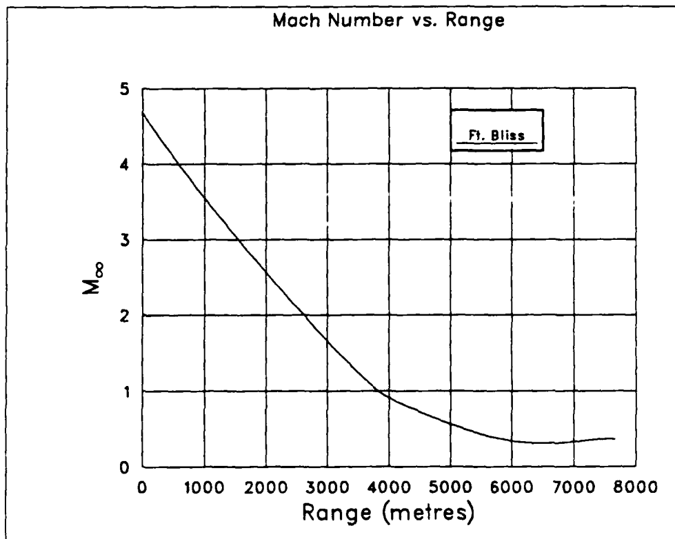
Figure (17) Ft. Bliss Trajectory: Mach Number versus Range
