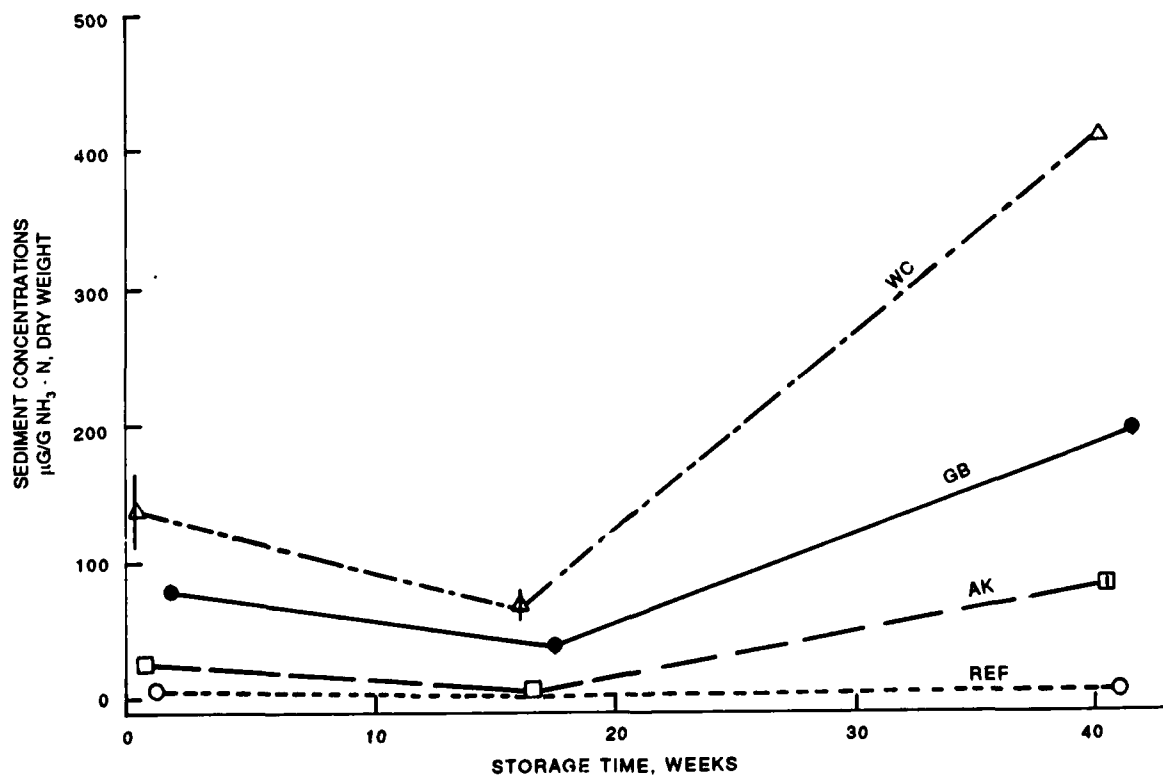
Figure 8. Results of sediment analyses for NH 3 -N (initial and at 16 and 40 weeks)
