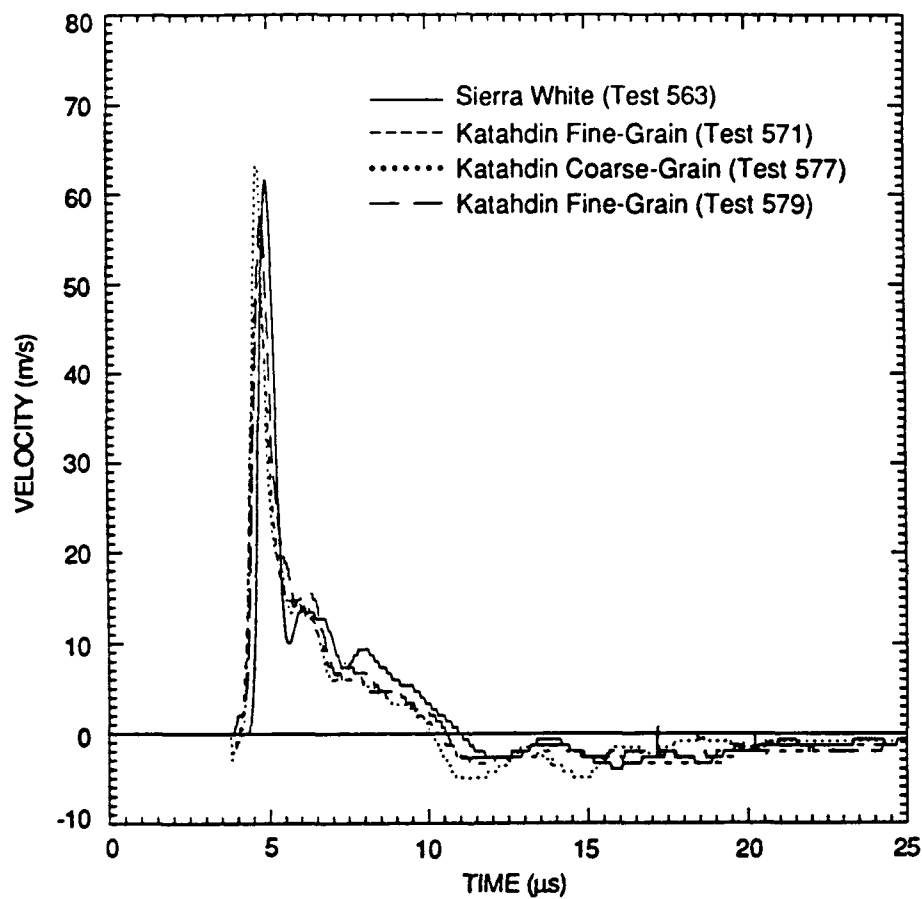
Figure 24. Particle velocity histories measured at 25-mm range in different types of granite.
