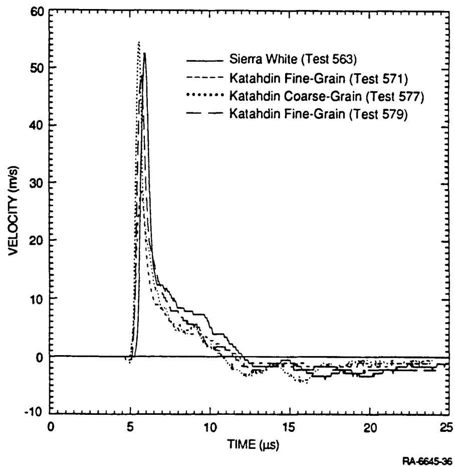
Figure 25. Particle velocity histories measured at 30-mm range in different types of granite.
