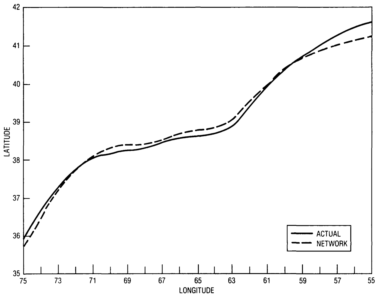
Figure 2. Proximity of 3 modes from grid-input or 2500-40-6 neural network (dashed line) to the actual 3 modes (solid line) for a test Gulf Stream.
