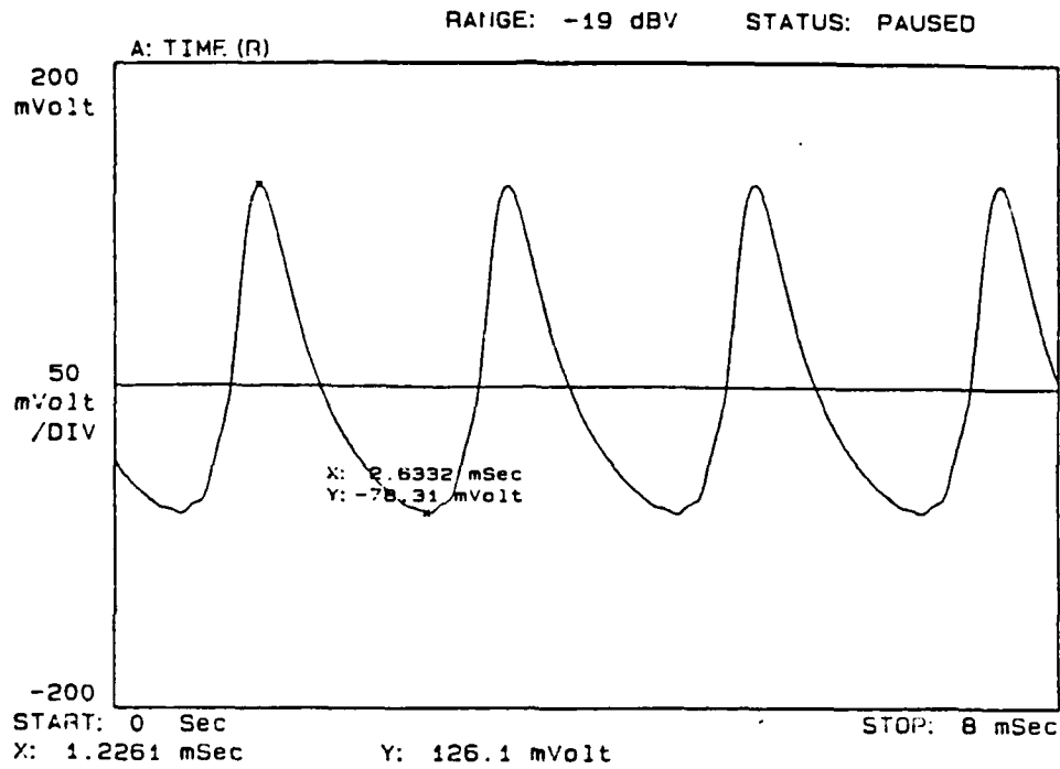
Figure 11: Waveform of the sound generated by the prime mover at a temperature difference of 368°C.
