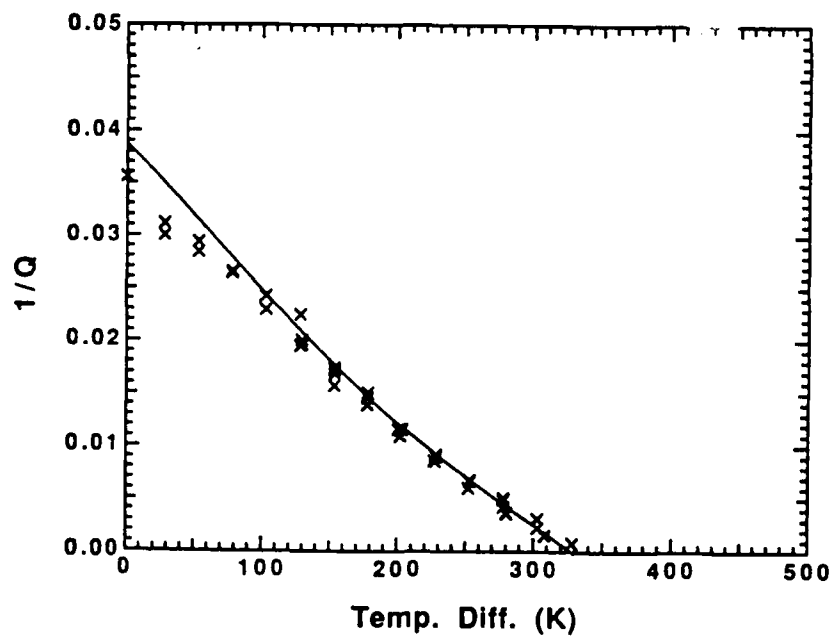
Figure 8: Graph of 1/Q vs the temperature difference across the prime mover stack filled with helium at a mean pressure of 238 kPa. The curve is the results of calculations discussed in Ref. 11.
