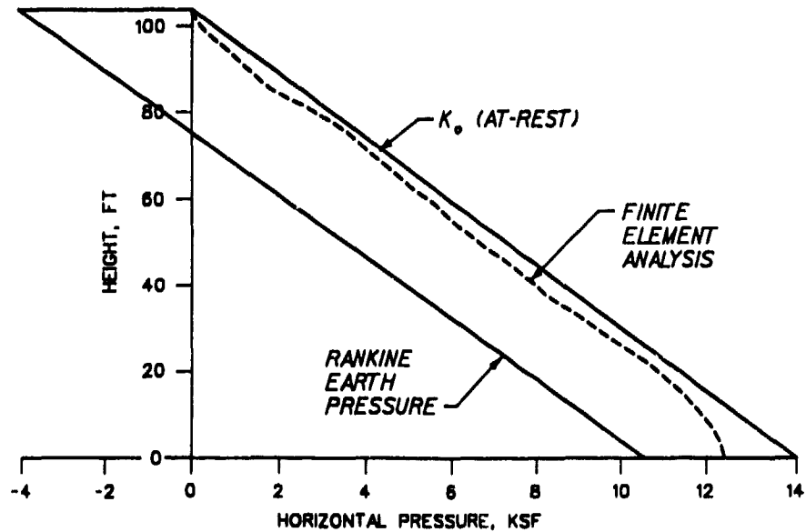
b. Soft core analysis
