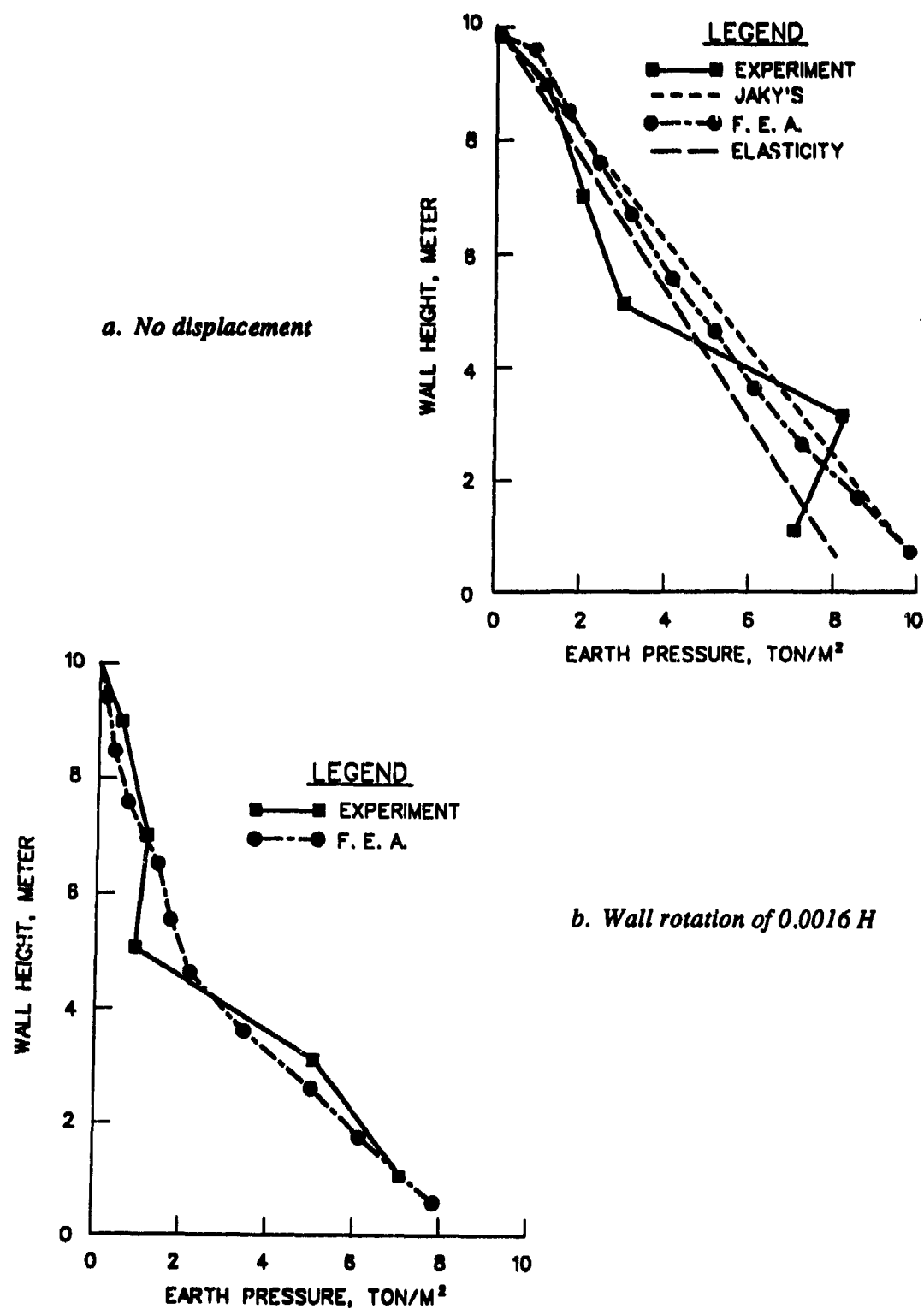
Figure 9. Earth pressure distribution in study by Bhatia and Bakeer (1989)
