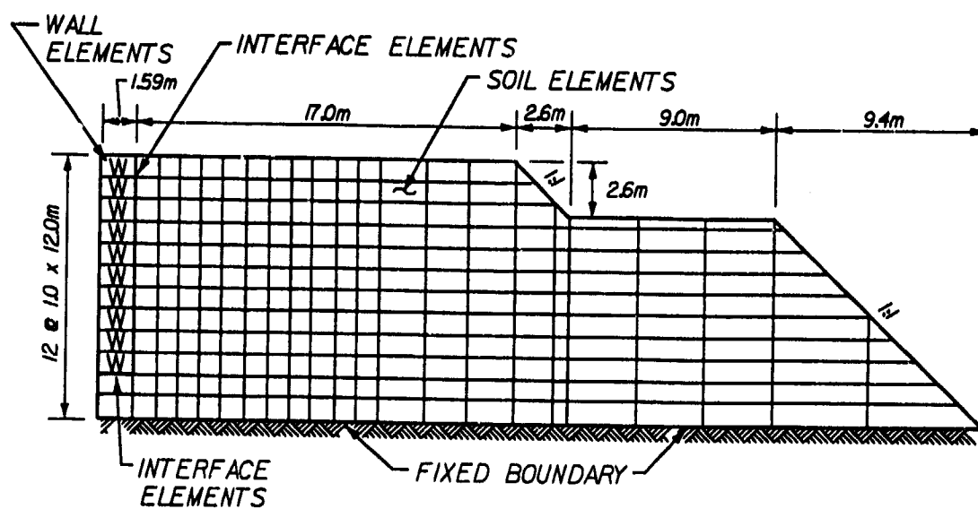
b. Basic finite element mesh
