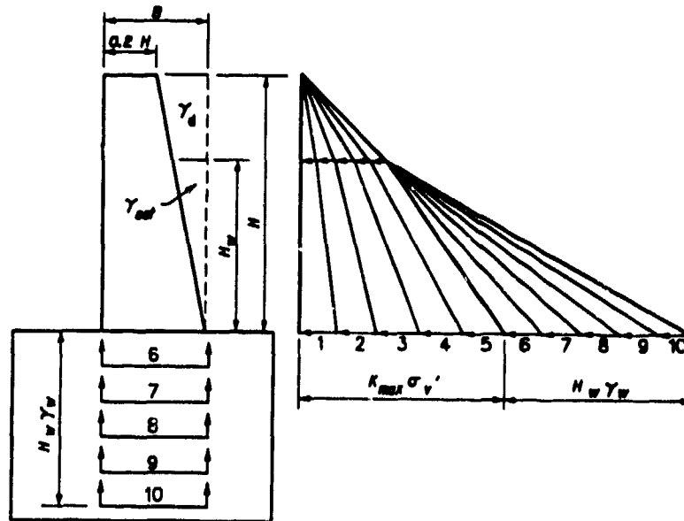
a. Incremental pressure applications used in following load analysis
