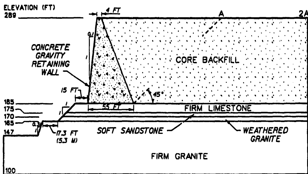
a. Wall modeled section
