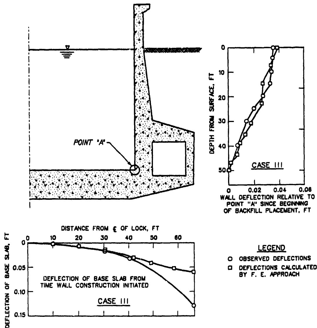
Figure 2. Structural deflections for Case III - Port Allen Lock (Clough and Duncan 1969)
