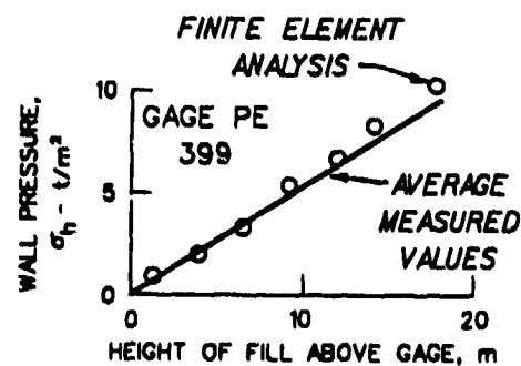
b. Results of nonlinear finite element calculations and gage PE 399 - during backfilling
