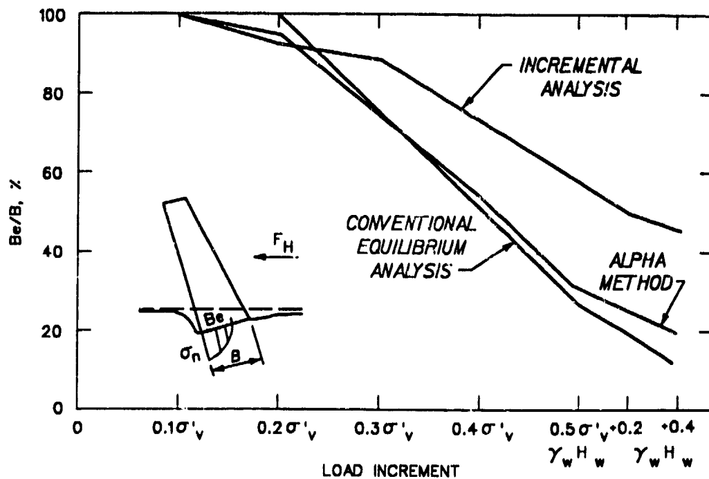
b. Variation of B_e/B with lateral load (Ebeling et al. 1988)
