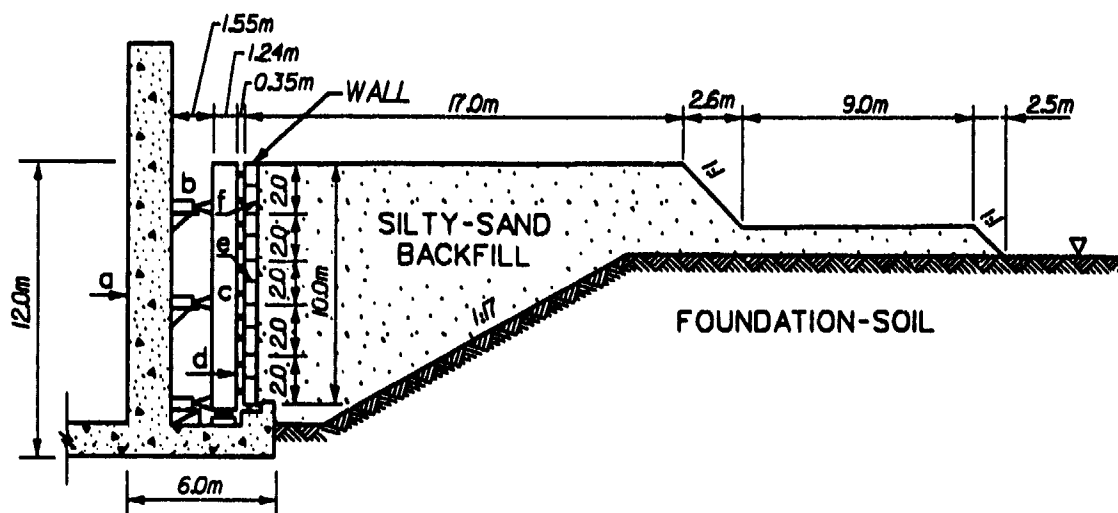
a. Experimental wall model
