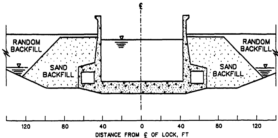
a. Cross section of Port Allen Lock
