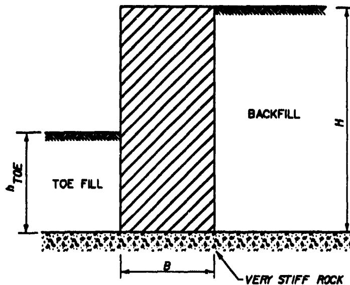
a. Rectangular hypothetical structure used in the backfill placement analysis
