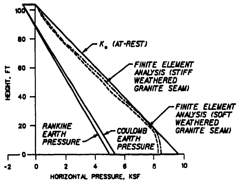
a. Stiff core analysis
