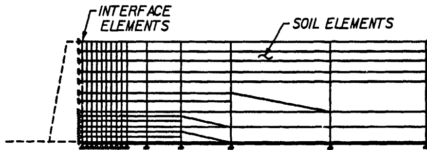
a. Retaining wall—backfill system
