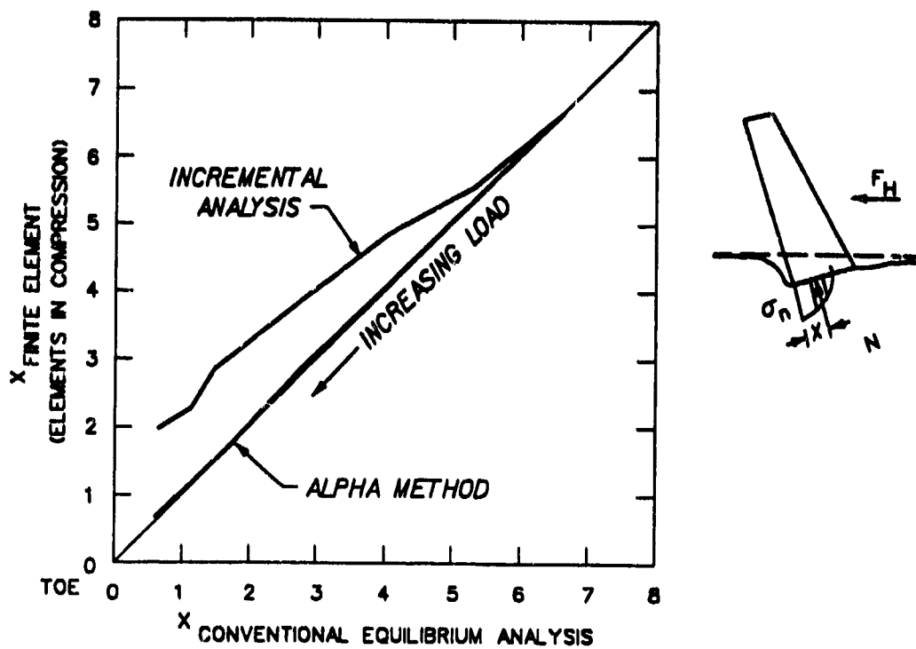
a. Location of resultant normal force as computed using finite element and conventional equilibrium methods
