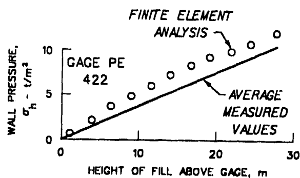
c. Results of nonlinear finite element calculations and gage PE 422 - during backfilling
