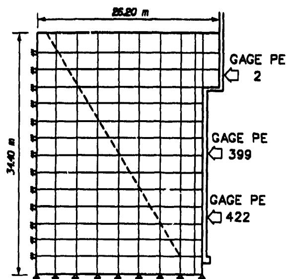
a. Cross section with finite element mesh and earth pressure cells
