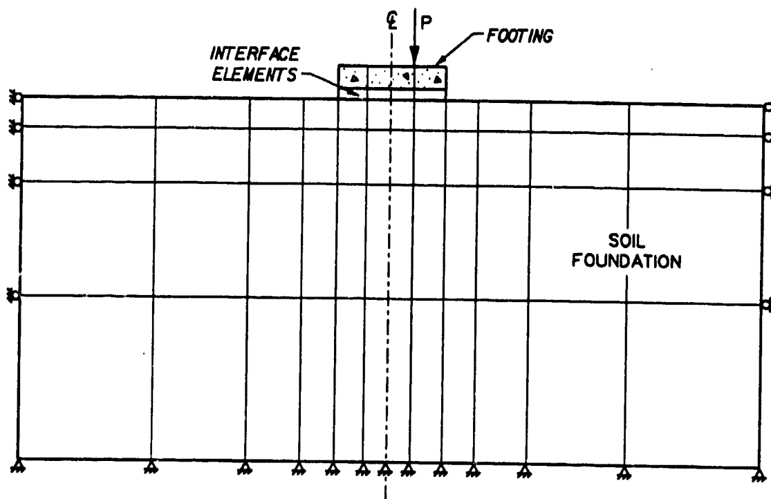
a. Finite element idealization of footing-soil continuum
