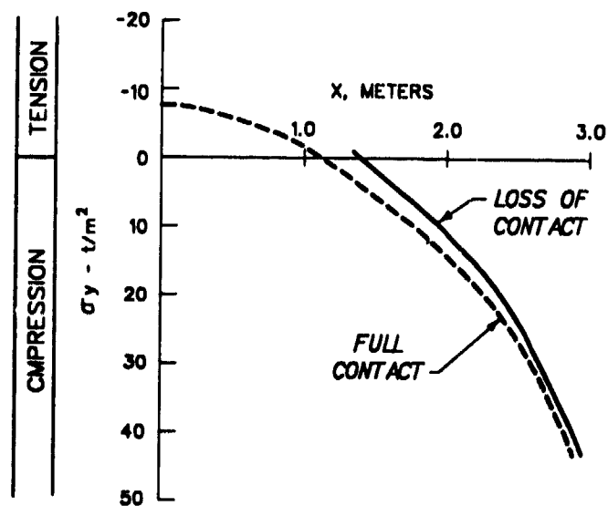
b. Contact stress distribution
