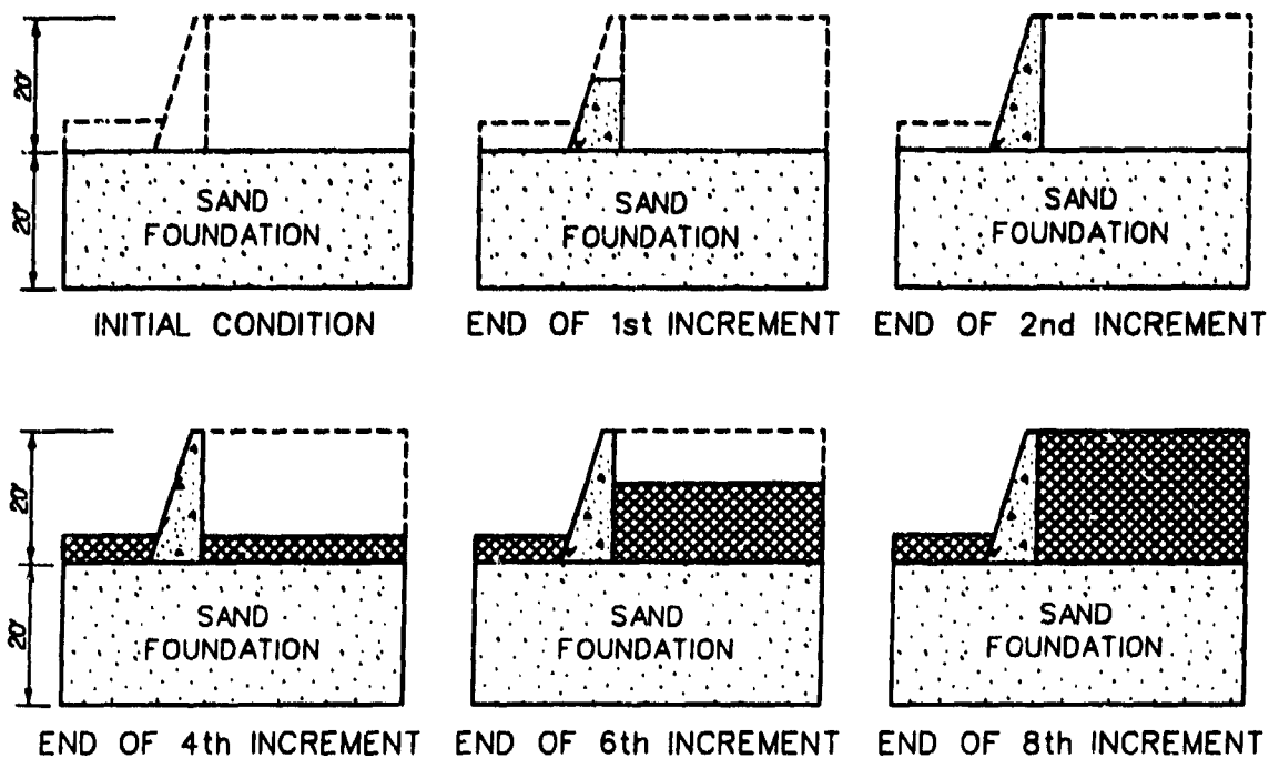
Figure 10. Gravity wall construction sequence (Clough and Duncan 1971)
