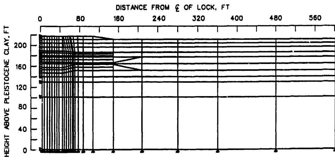
b. Finite element mesh employed for incremental analyses of Port Allen Lock
