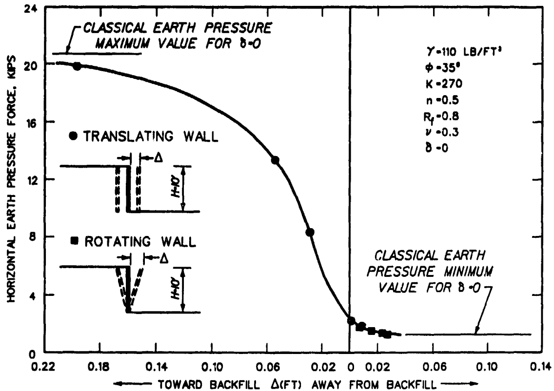
Figure 7. Variations of earth pressure force with wall movement calculated by finite element analyses (Clough and Duncan 1971)
