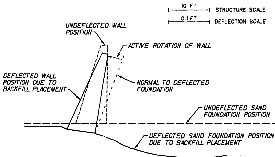
Figure 11. Wall and sand foundation deflections during backfill placement
