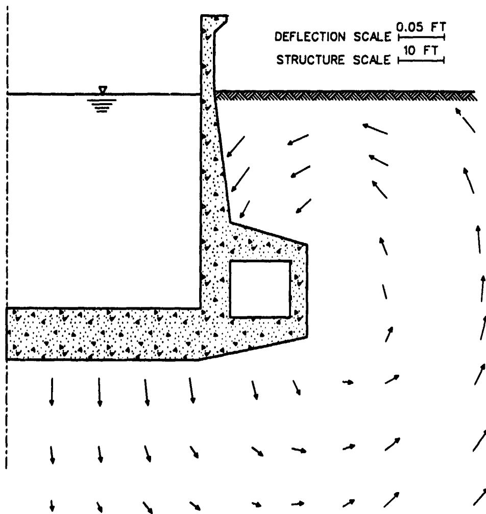
Figure 5. Calculated movements due to filling Port Allen Lock with water (Clough and Duncan 1969)
