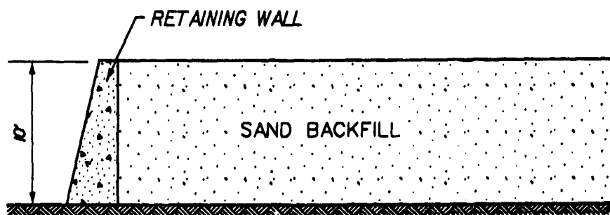
b. Retaining wall—finite element representation
