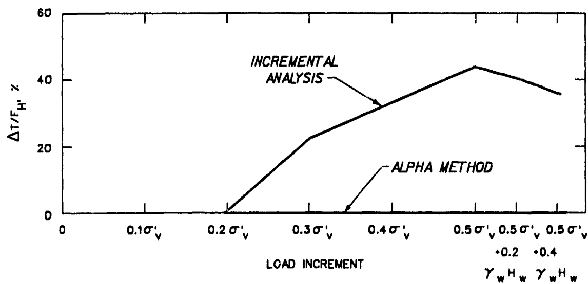
Figure 23. Development of overshoot forces with lateral load (Ebeling et al. 1988)
