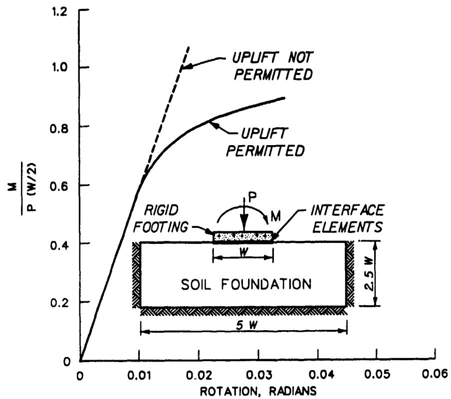
Figure 20. Moment-rotation relationship for footing (Herrmann 1978)
