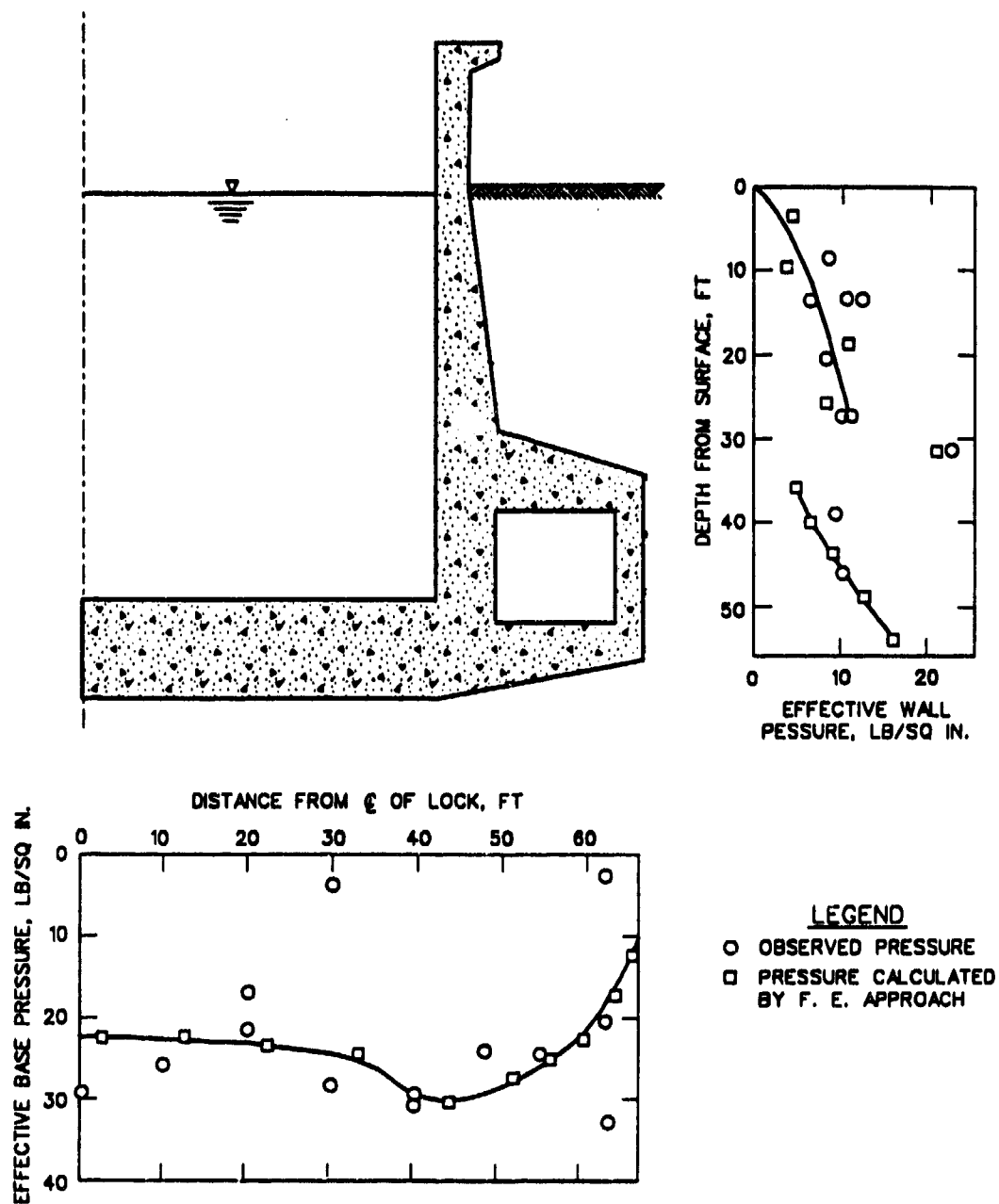
Figure 3. Effective earth pressures for Case III - Port Allen Lock (Clough and Duncan 1969)
