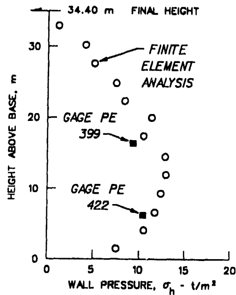
d. Results of nonlinear finite element calculations and gages PE 399 and PE 422 - after backfilling
