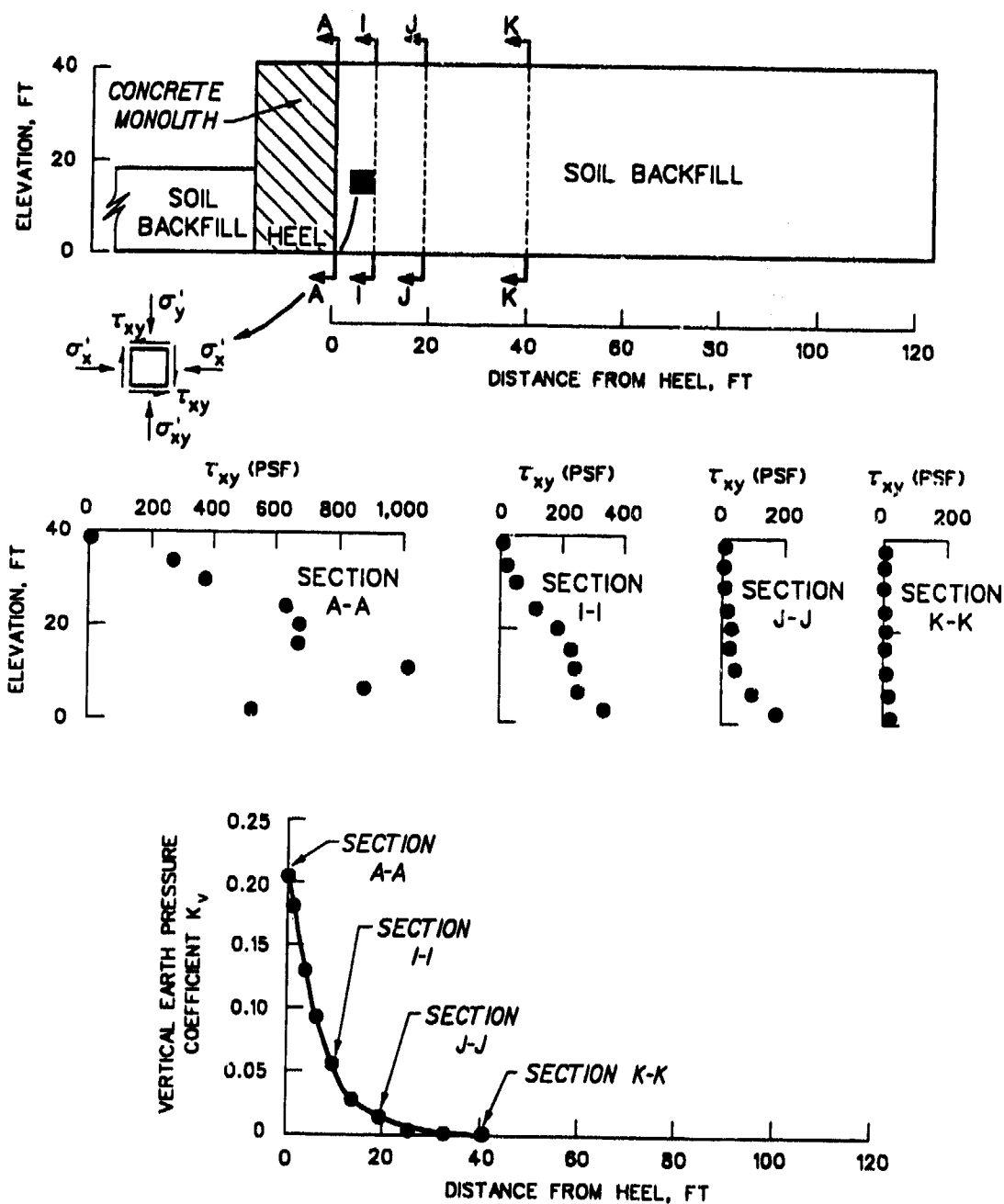
Figure 17. Variation of distribution of shear stress and vertical earth pressure coefficient with distance from the heel of the wall (Ebeling, Duncan, and Clough 1989)
