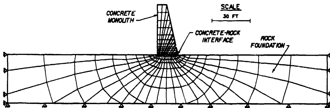
b. Fine finite element mesh used to model the base case hypothetical structure
