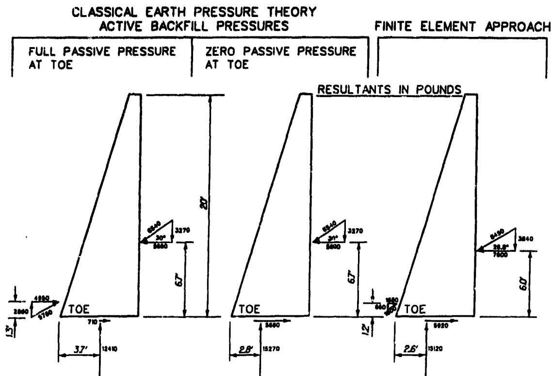
Figure 12. Earth pressure resultants acting on wall from classical earth pressure theory and finite element results (Clough and Duncan 1971)
