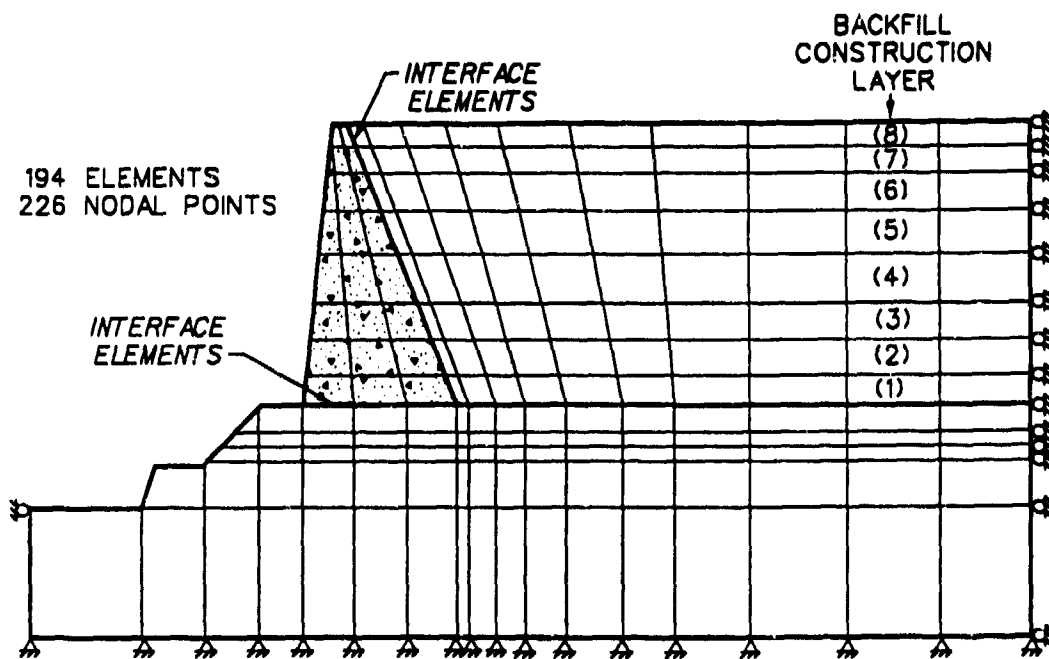
b. Finite element mesh for wall
