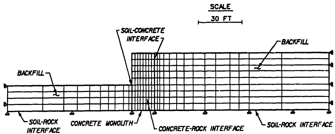
b. Finite element mesh used to model a rectangular hypothetical structure with additional backfill beyond the toe
