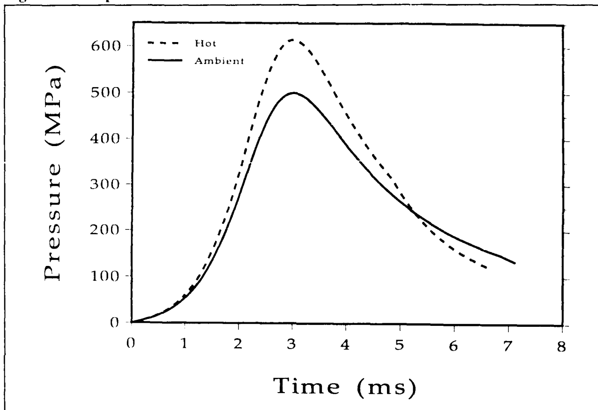
Figure 1. Temperature-Induced Breech Pressure Differences.
