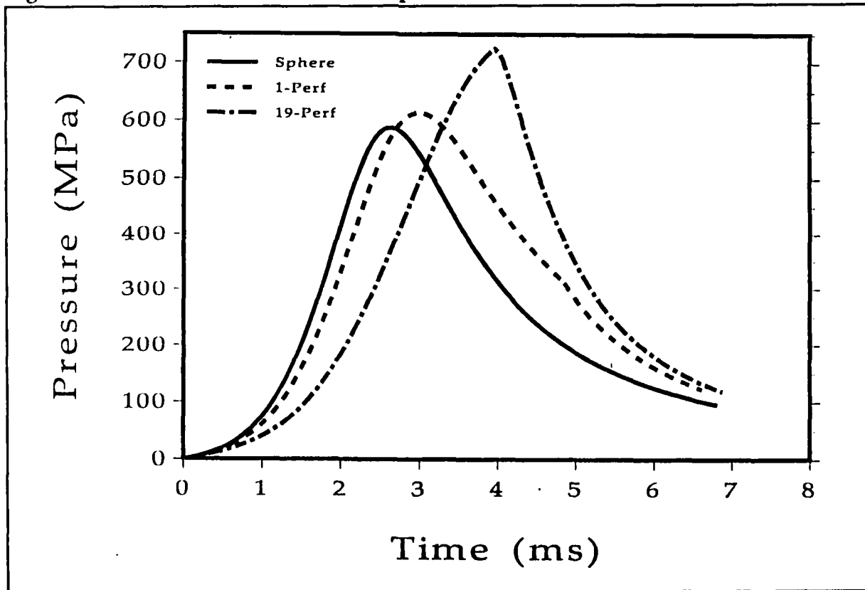
Figure 3. Breech Pressures at Hot Temperature.
