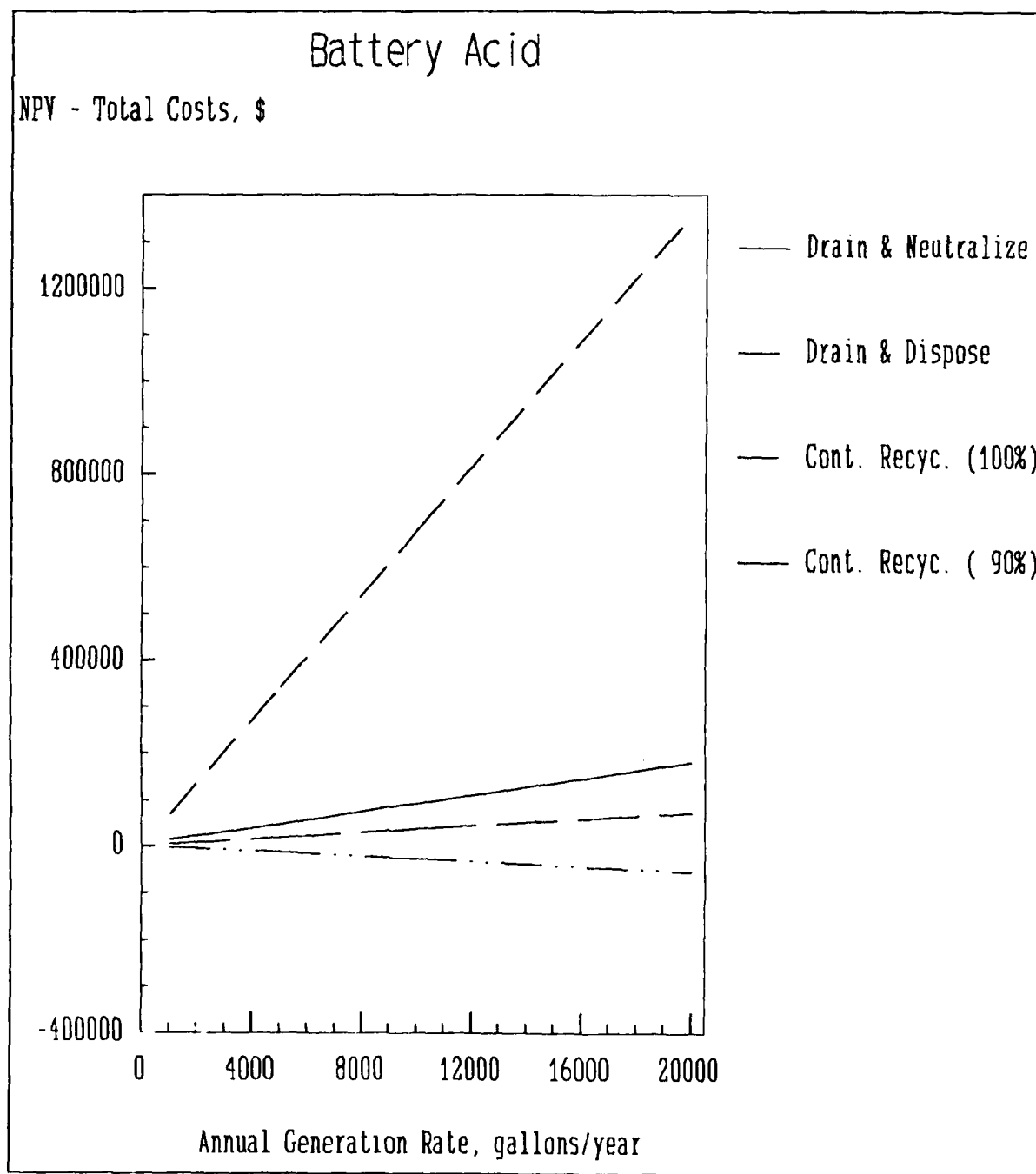
Figure 8. Comparison of the NPVs of the total 10-yr costs for implementing options for the minimization of spent battery acid. Draining and neutralization define the status quo.
