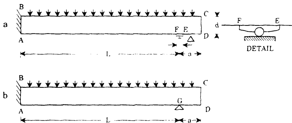
Fig.2.1 The simply supported cantilever beam
