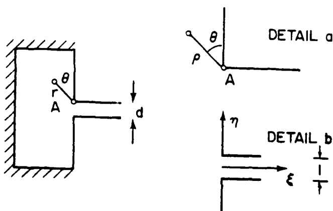
Fig.4.2. The solution on the zoomed domain.
