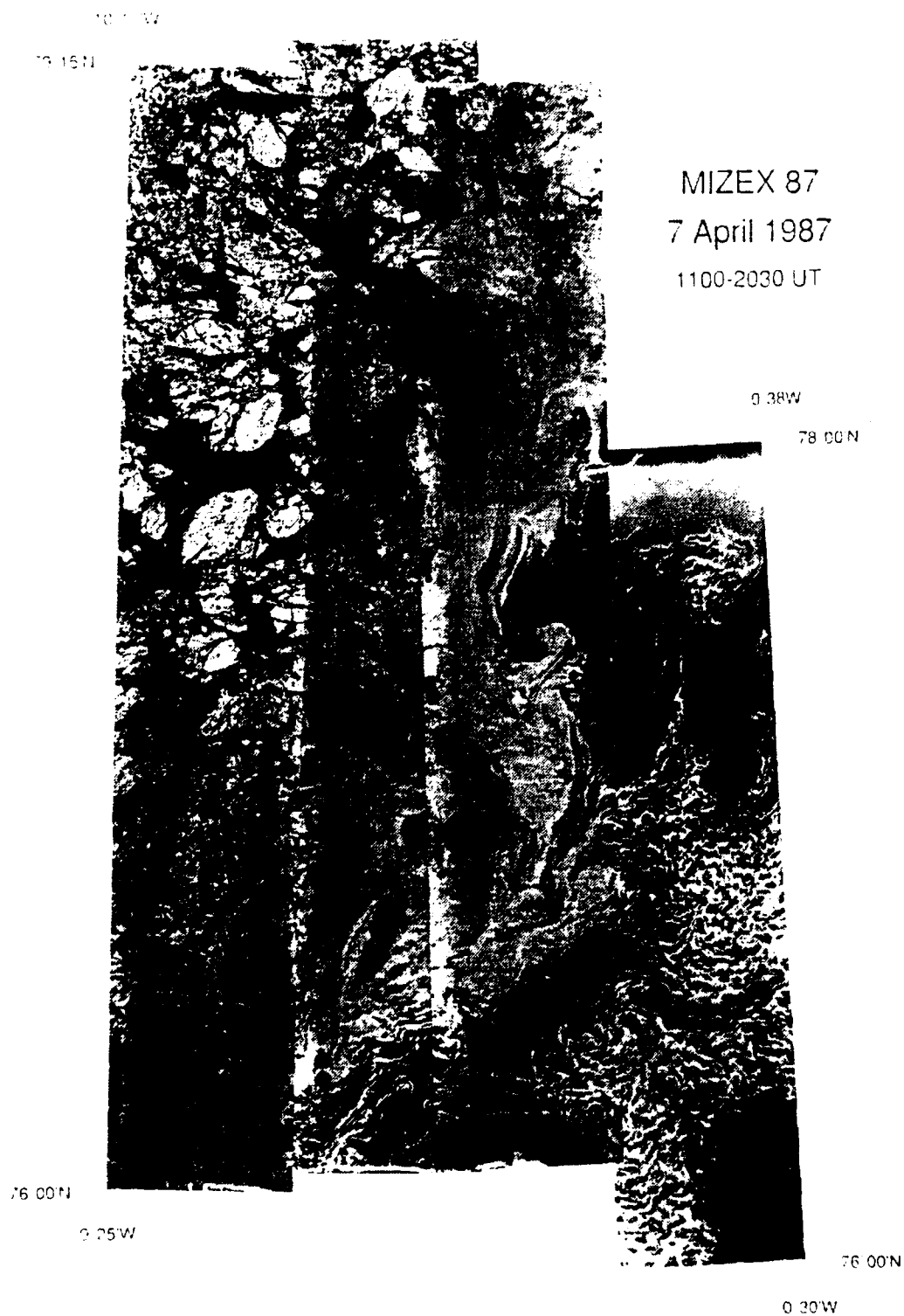
Figure 18. SAR image mosaic from mission 16 [from Shuchman et al., 1988].
