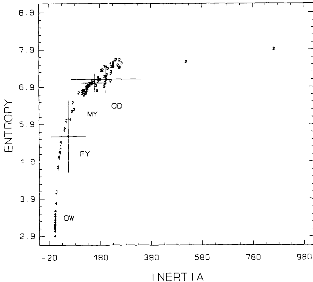
1=FY, 2=MY, 3=OD, 4=OW Figure 38. Plot of top two texture statistics, inertia and entropy, from the original data set indicates good discrimination using only two statistics for OW and FY but not for MY and OD.
