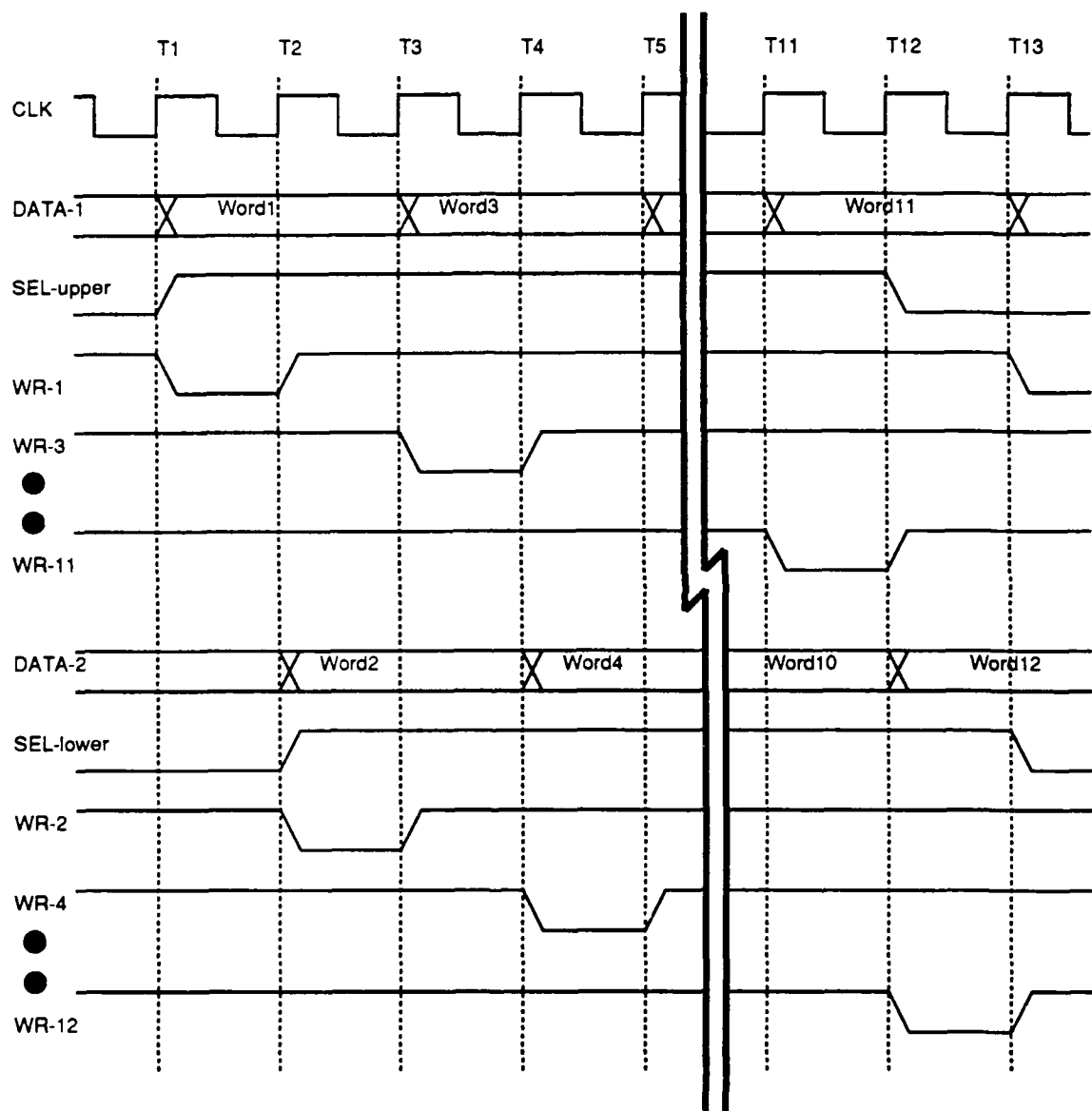
Figure 3.4: Writing into a Packet Buffer
