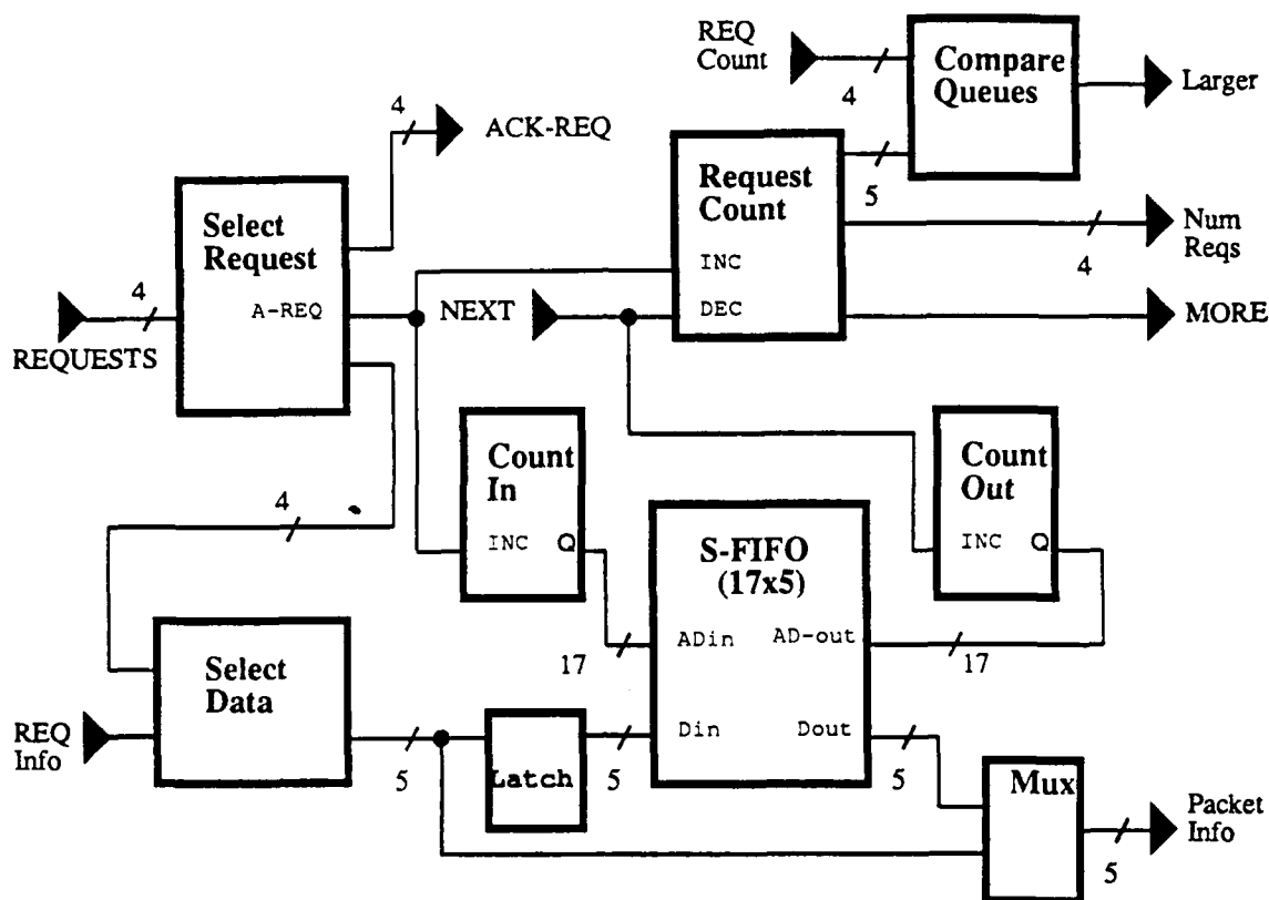
Figure 3.5: Block Diagram of the Scheduler
