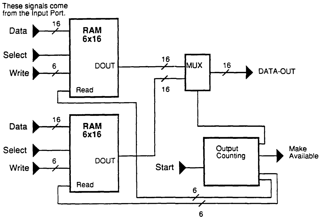
Figure 3.1: A Packet Buffer
