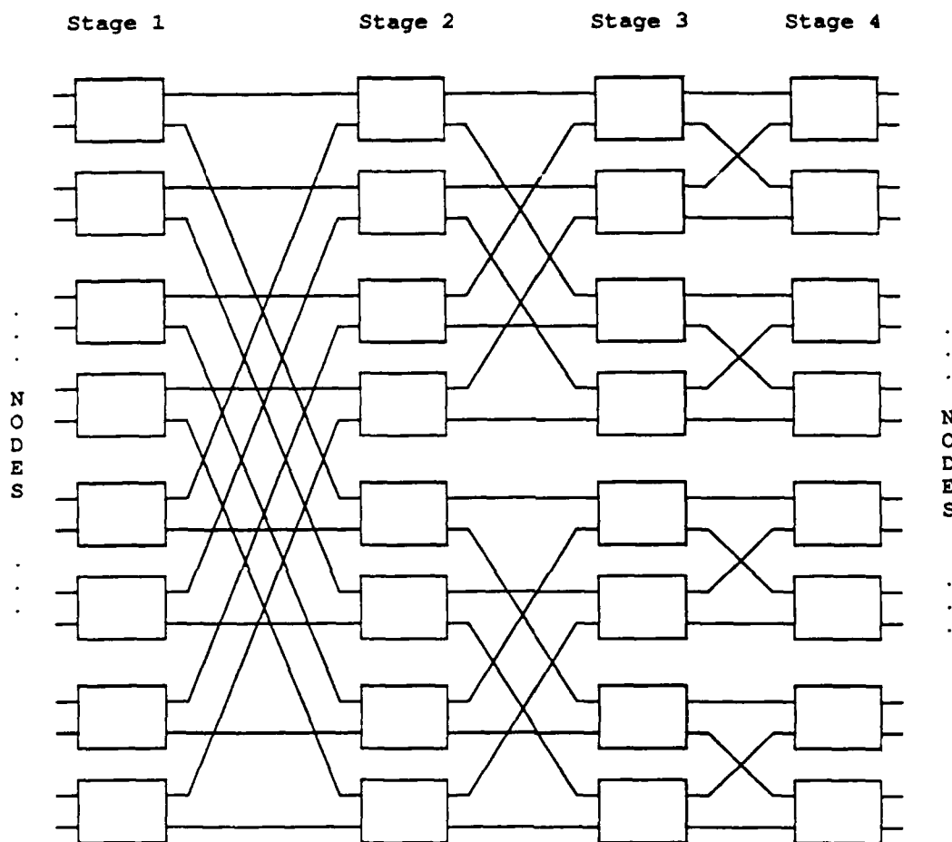
Figure 1.1: A Butterfly Network using 2 \times 2 Switches.
