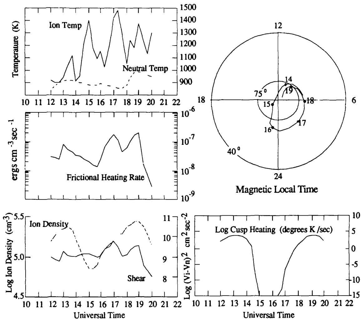
Figure 4.3 Summary plot of a flux tube convection path and frictional heating history taken from the TIGCM solution fields near 200 km. A flux tube trajectory is selected which is at or near the location of the upwelling ion event (UWI) observed by DE-1. The three-dimensional heating history of this flux tube is consolidated from the TIGCM solutions and is used as a time-dependent input to the polar wind model. Strong low altitude ion heating near 19 UT generated a transient upwelling of O + .
