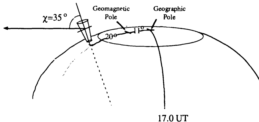
Figure 3.1 A flux tube located near 70^\circ N 00^\circ W geomagnetic experiences the greatest amount of EUV flux near 17 UT (12 MLT) at summer solstice due to the relative positions of the geographic and geomagnetic poles.
