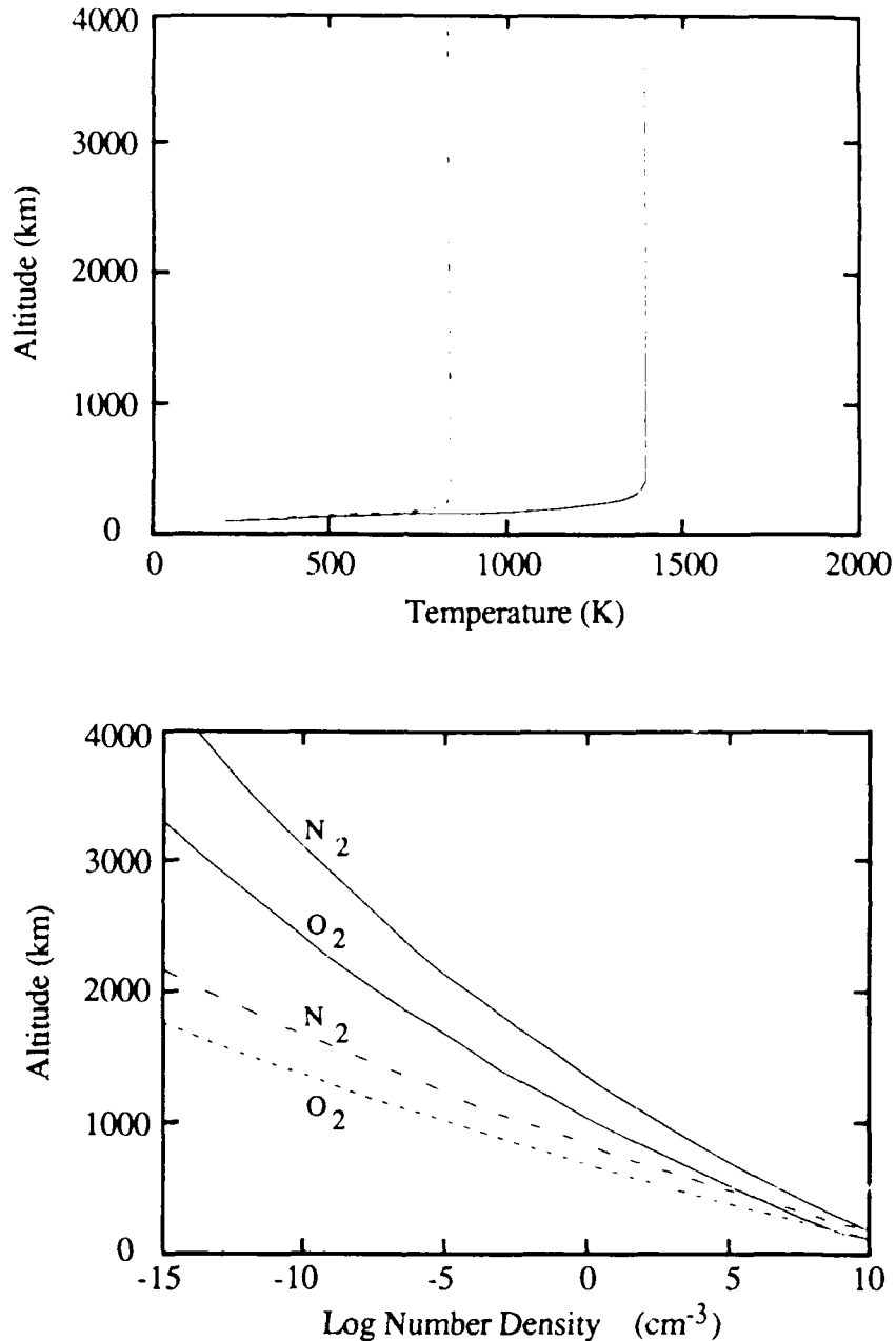
Figure 3.3 Number density profiles of molecular nitrogen and oxygen (b) derived from MSIS-86 for 80^\circ \text{N} 00^\circ \text{W} geomagnetic at 12 MLT for solar minimum (dashed) and maximum (solid). Number density enhancements for both species occur for the solar maximum case due to higher Thermospheric temperatures(a).
