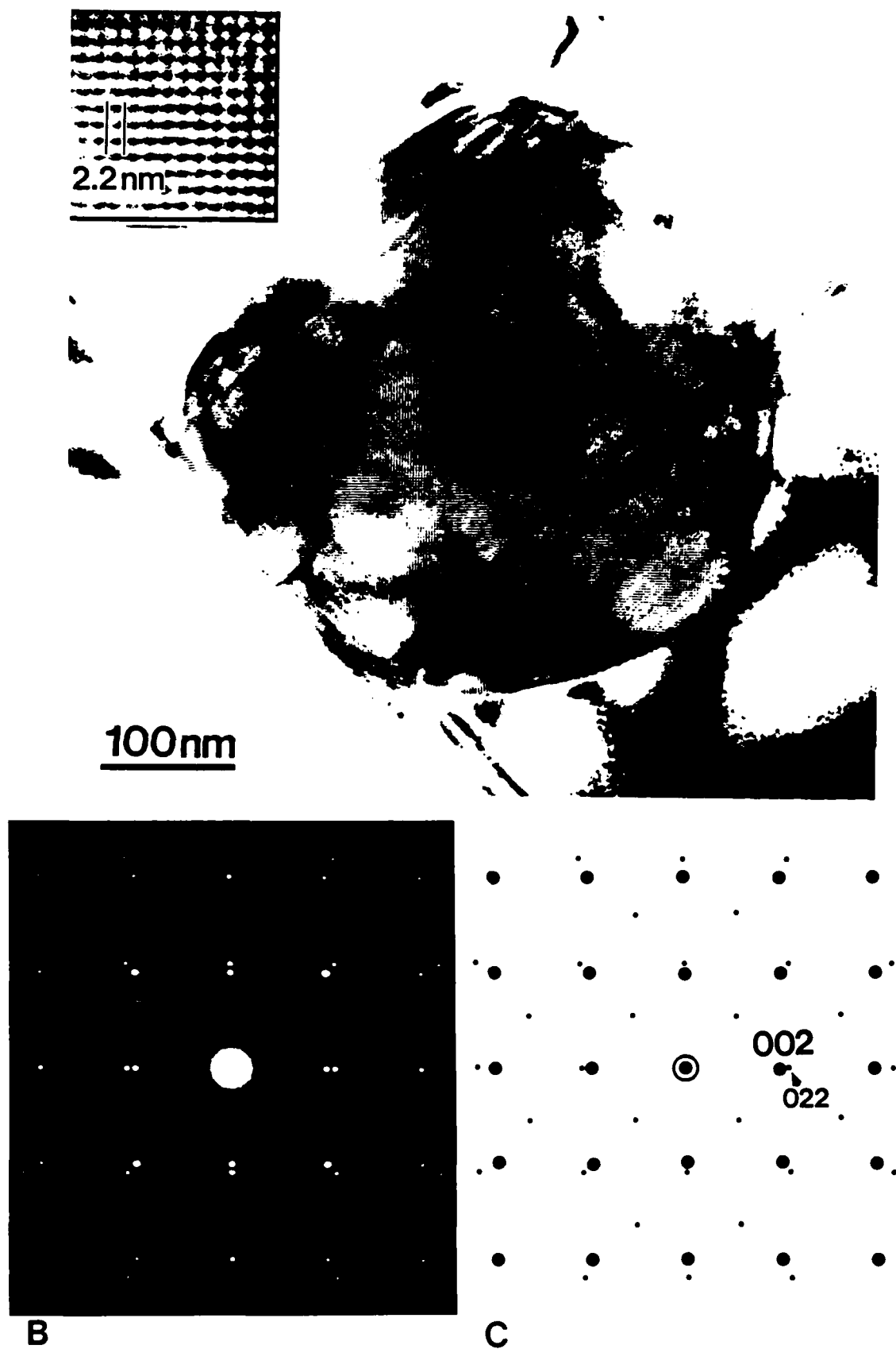
Fig.17 ThO 2 particle on (100) β-SiC surface. A.) BF image , B.) corresponding SAD pattern and C.) schematic diagram which shows (002) β-SiC ∥ (022) ThO 2 with [100] β-SiC ∥ [100] ThO 2 . Moiré fringe periodicity in "A" (2.16nm) consistent with 9.3% lattice misfit.
