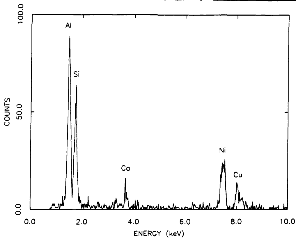
Fig.23 Contaminated thin-film reaction couple. A.) BF image showing light-shaded siliceous layer between NiAl 2 O 4 particles and \alpha -Al 2 O 3 substrate, B.) EDS spectrum recorded from contamination layer showing presence of Si and Ca impurities.
