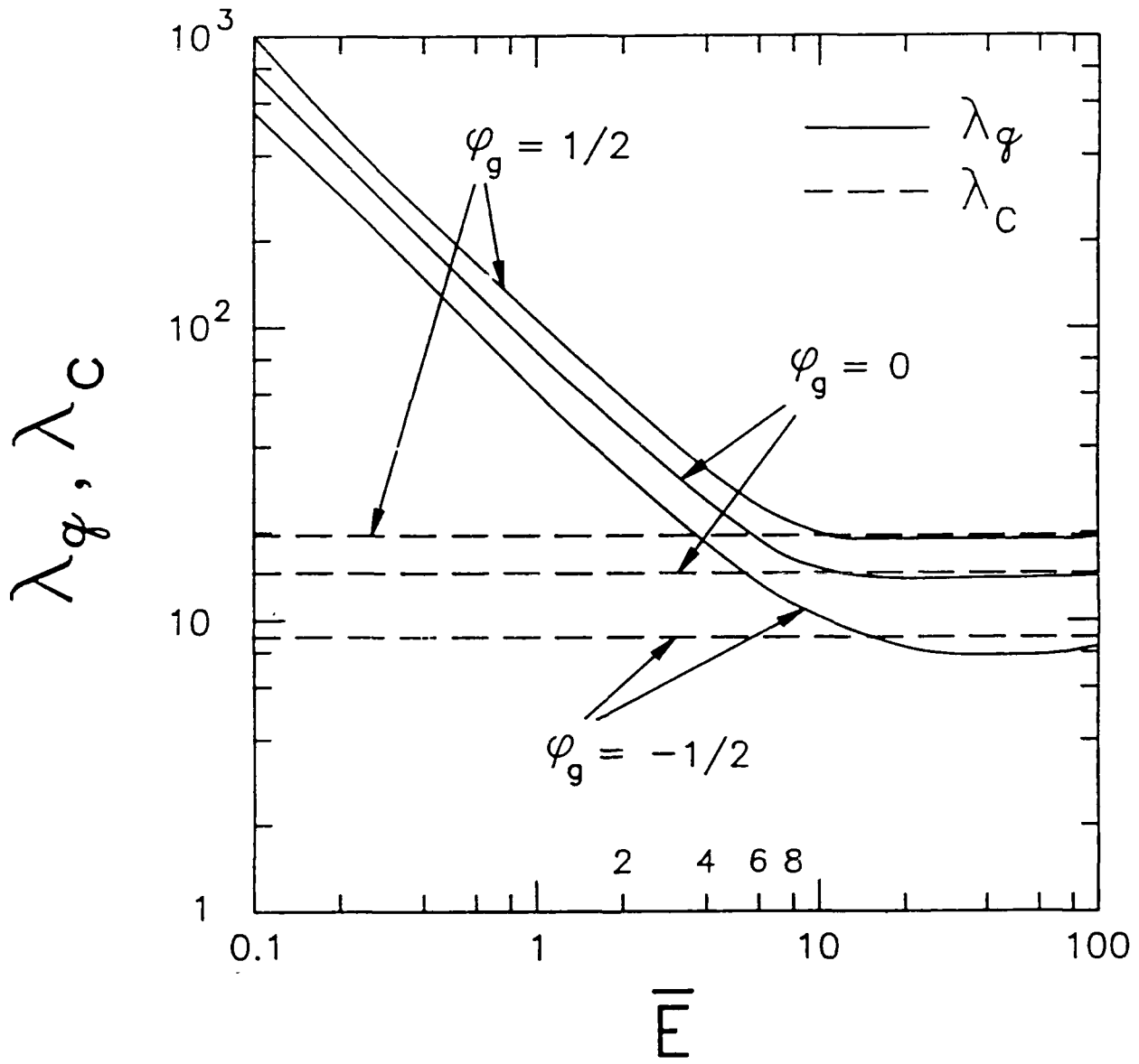
Fig. 1 — The solid curves show the normalized critical current ( \lambda_q ) as a function of \bar{E} for \phi_g = 0, \pm 1/2 . The classical values ( \lambda_c ) are indicated by the dotted lines.
