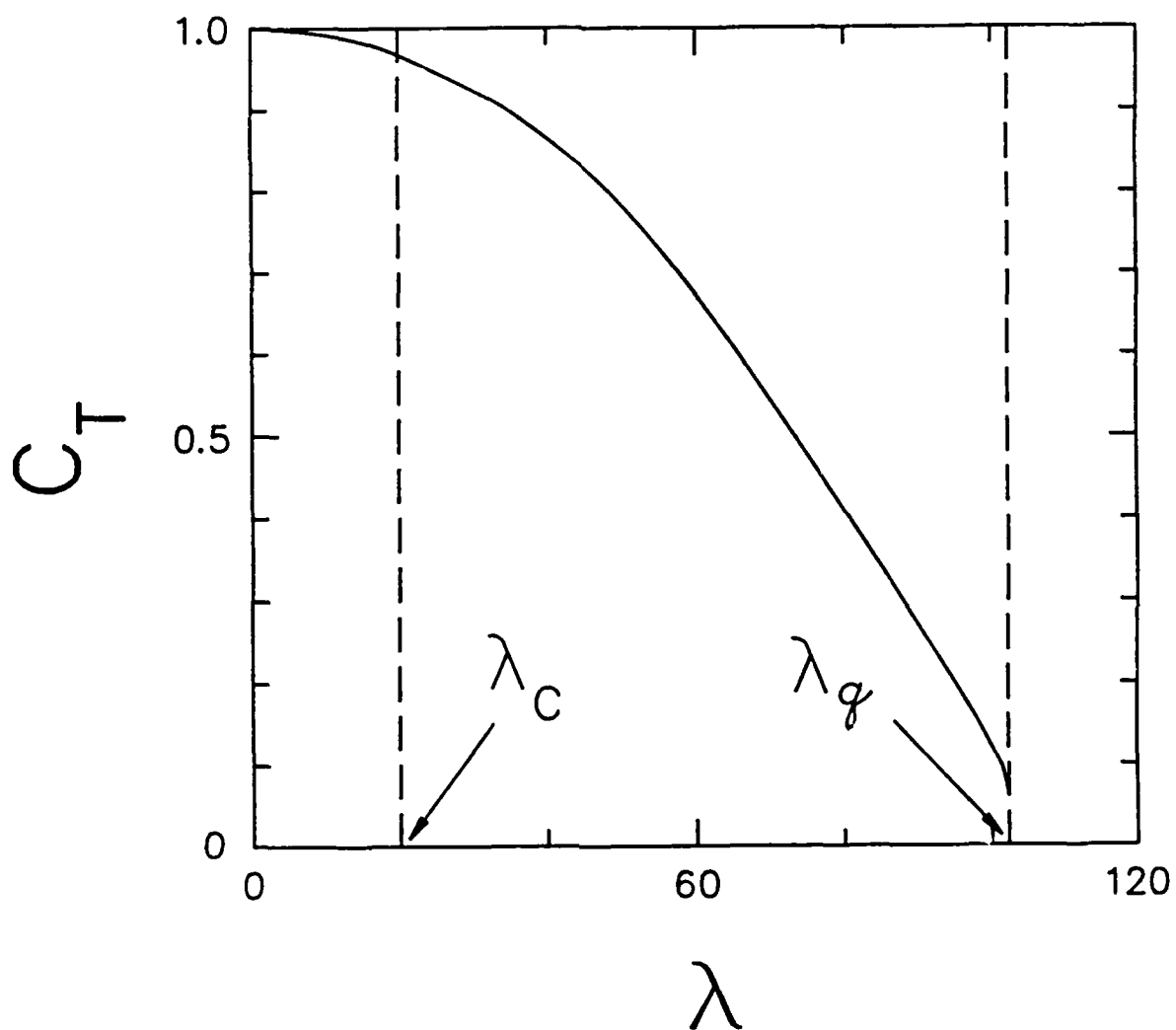
Fig. 3 — The transmission coefficient C_T as a function of \lambda for \bar{E} = 1 , \phi_g = 0.5 . The values of \lambda_g and \lambda_c are indicated by the dotted lines.
