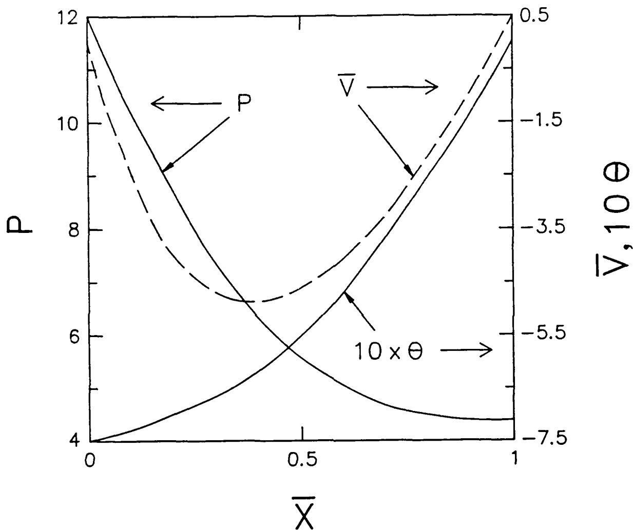
Fig. 2 — The solutions p , \theta and \bar{V} for the case \bar{E} = 1 , \lambda = 95 , and \phi_s = 0.5 . Tunneling effects are apparent as \bar{E} + \bar{V} < 0 over a wide range of \bar{x} .
