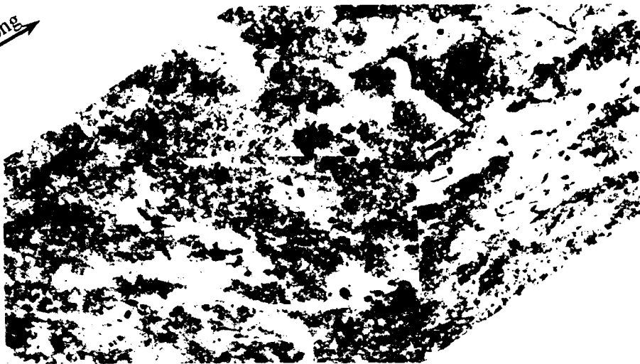
Figure 11. F/A-18 FT40 in flange region of plate has a structure similar to that of the previous sample. The main difference appears to be in the size and number of the large precipitates that are mainly centred in the regions of the large grains. These precipitates appear to be both more numerous and generally slightly larger than those of the previous sample.
