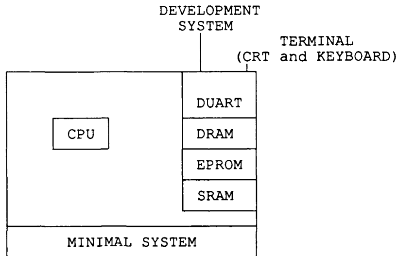
Figure 4.1: Minimal System
