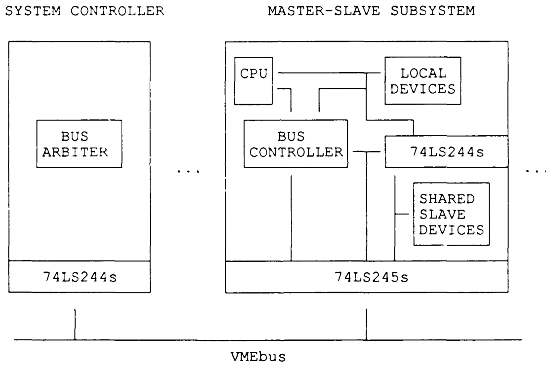
Figure 2.3: Master-Slave Subsystem
